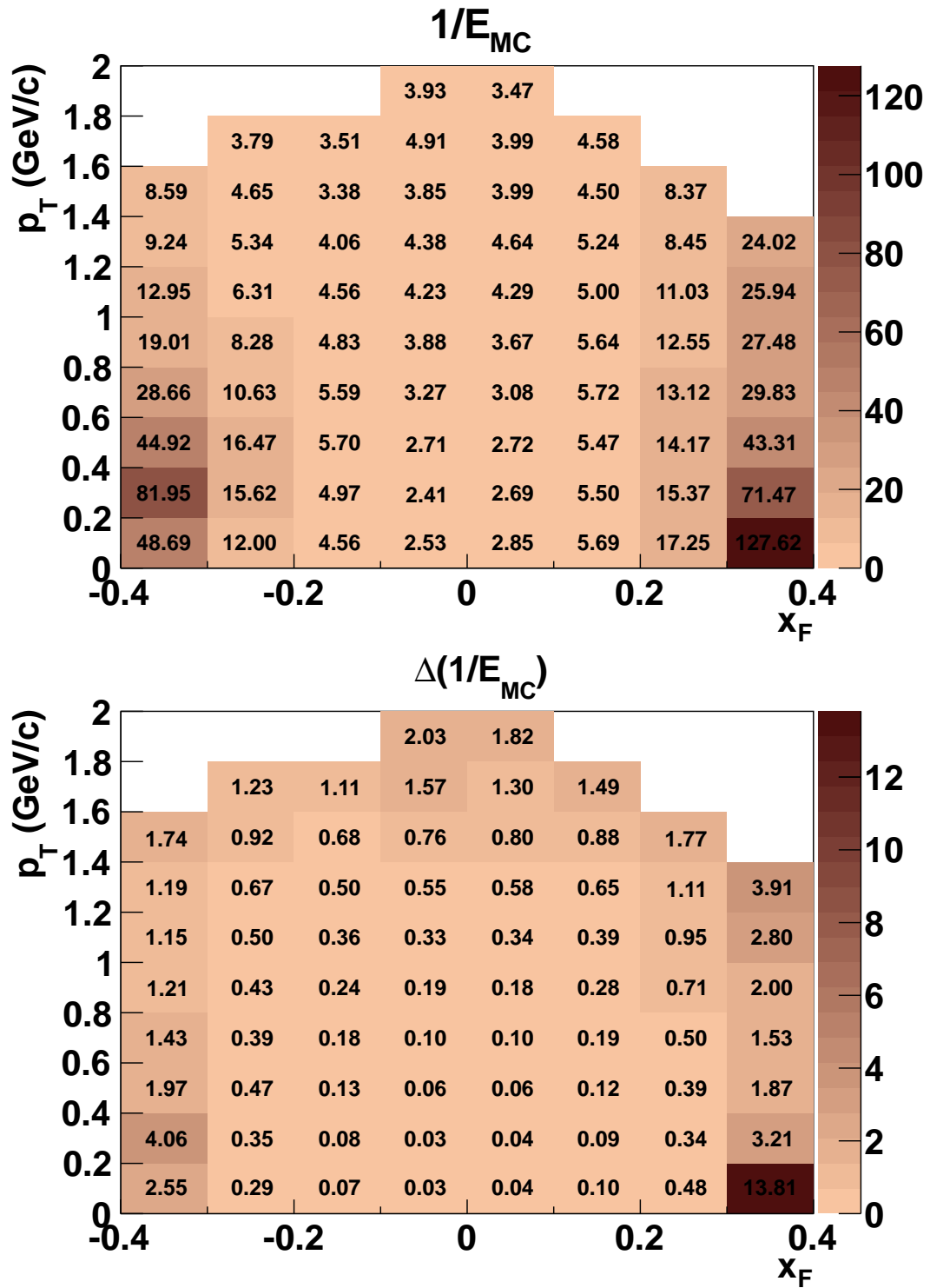
Figure C.18. Top : MC-correction factor 1/E_{MC} . Bottom : Statistical error of the correction factor \Delta(1/E_{MC}) .
