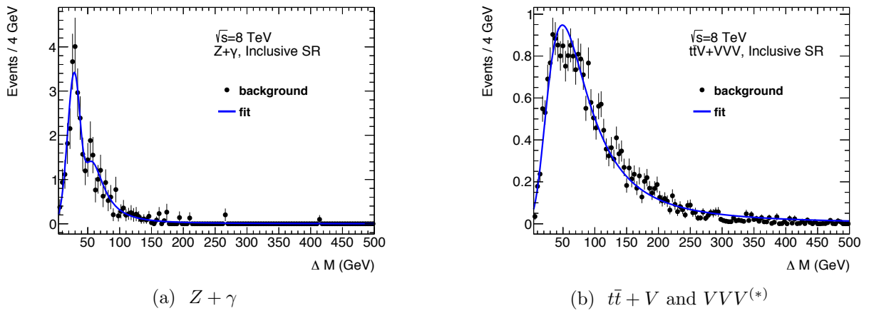
Figure 8.23: \Delta m distributions from Monte Carlo and Landau function fits for the Z + \gamma (left) and t\bar{t} + V plus VVV^{(*)} (right) backgrounds. For the Z + \gamma background, the inclusive, Z + e signal region is shown; the background is negligible in the Z + \mu signal regions. For the t\bar{t} + V plus VVV^{(*)} backgrounds, the inclusive signal region is shown, with the Z + e and Z + \mu channels combined.
