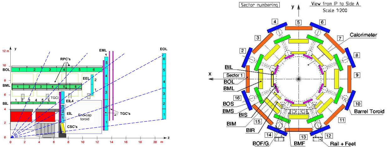
(a) R-z view of the muon spectrometer barrel. The barrel contains three layers, each with eight large and eight small chambers.
