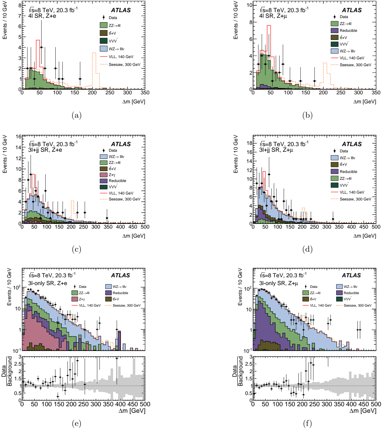
Figure 8.24: The \Delta m distributions for the 4\ell (top), 3\ell + jj (middle), and 3\ell -only (bottom) categories, divided into the Z + e (left) and Z + \mu (right) flavor channels. The data are shown as black points, while the pre-fit background expectations are shown in the solid histograms. Signal contributions from a 140 GeV L^\pm in the VLL model and a 300 GeV L^\pm in the seesaw model are also shown. The error bars on the points represent statistical uncertainties, and the shaded bands represent the systematic uncertainties on the background predictions.
