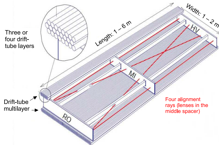
Figure 3.27: The mechanical structure of a MDT chamber. Two multilayers, each consisting of three or four rows of drift tubes, are separated by aluminum spacers. Four optical alignment rays continuously monitor the geometry of the chamber.
