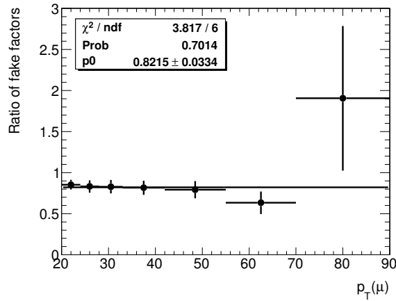
Figure 6.8: Ratio between the fake factors for muons with |d_0|/\sigma(d_0) > 3 compared to fake factors with nominal numerator and denominator definitions. These fake factors are derived from a POWHEG t\bar{t} sample.
