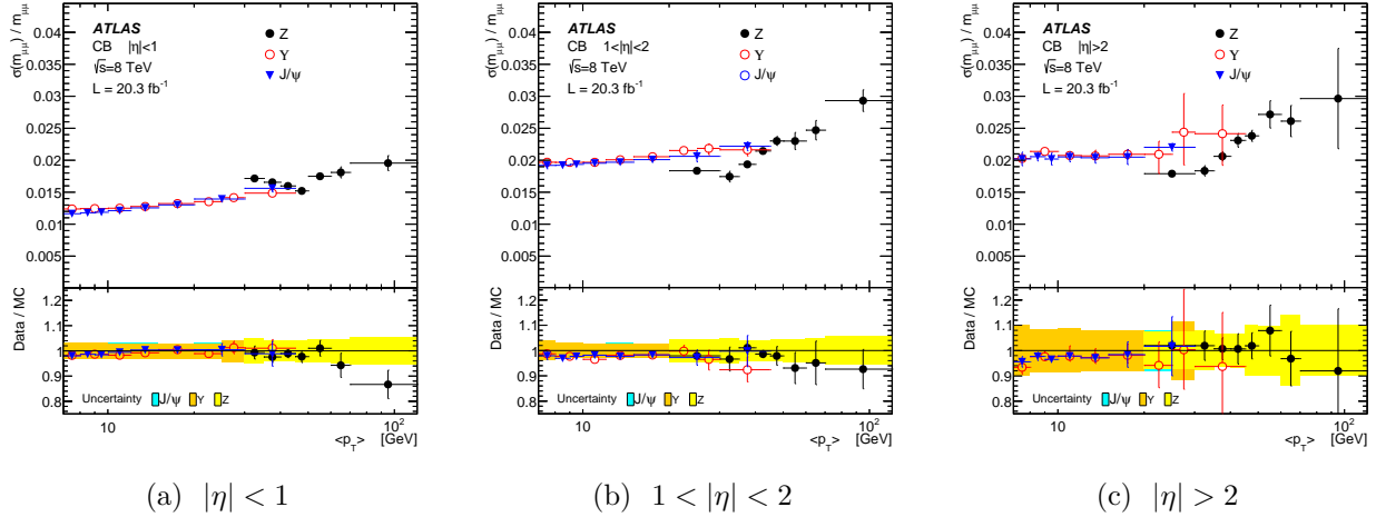
Figure 5.5: Dimuon invariant mass resolution for combined muons as a function of the average muon p_T in three pseudorapidity regions. The resolution is determined from J/\Psi \rightarrow \mu\mu , \Upsilon \rightarrow \mu\mu , and Z \rightarrow \mu\mu events. Both muons are required to be in the same pseudorapidity region. The J/\Psi and \Upsilon data are plotted as a function of \bar{p}_T = \frac{p_{T1} + p_{T2}}{2} , while Z data are plotted as a function of p_T^* = m_Z \sqrt{\frac{\sin \theta_1 \sin \theta_2}{2(1 - \cos \alpha_{12})}} , where \theta_{1,2} are the polar angles of the two muons and \alpha_{12} is the angle between the two muons, which removes the correlation between m_{\mu\mu} and \bar{p}_T . The lower panels show the ratio between data and the corrected MC, with bands representing the uncertainty on the MC corrections for the three calibration samples.
