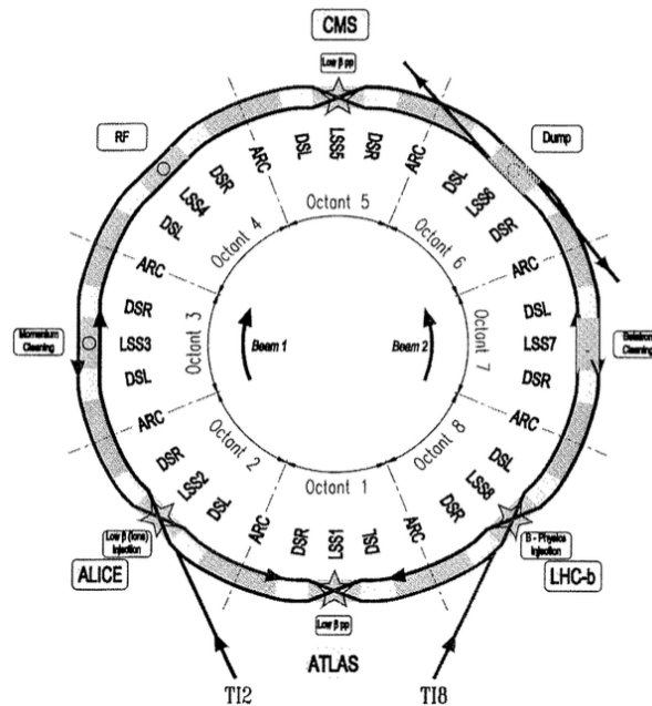
Figure 3.4: Layout of the LHC. The ring consists of eight arcs and eight long straight sections (LSS). Each junction between an arc and a LSS contains a dispersion suppressor cell (DSL, DSR). TI2 and TI8 are the two injection tunnels (“tunnel d’injection”) leading from the SPS to the LHC.
