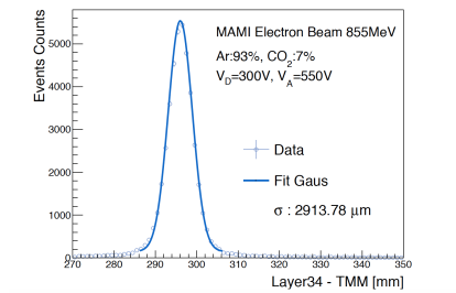
Figure 9: Difference between the cluster position calculated combining the stereo layer information and the measurement provided by the tracking chamber
