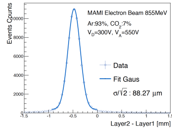
Figure 8: Difference between cluster position measured on the two sides of a readout panel
