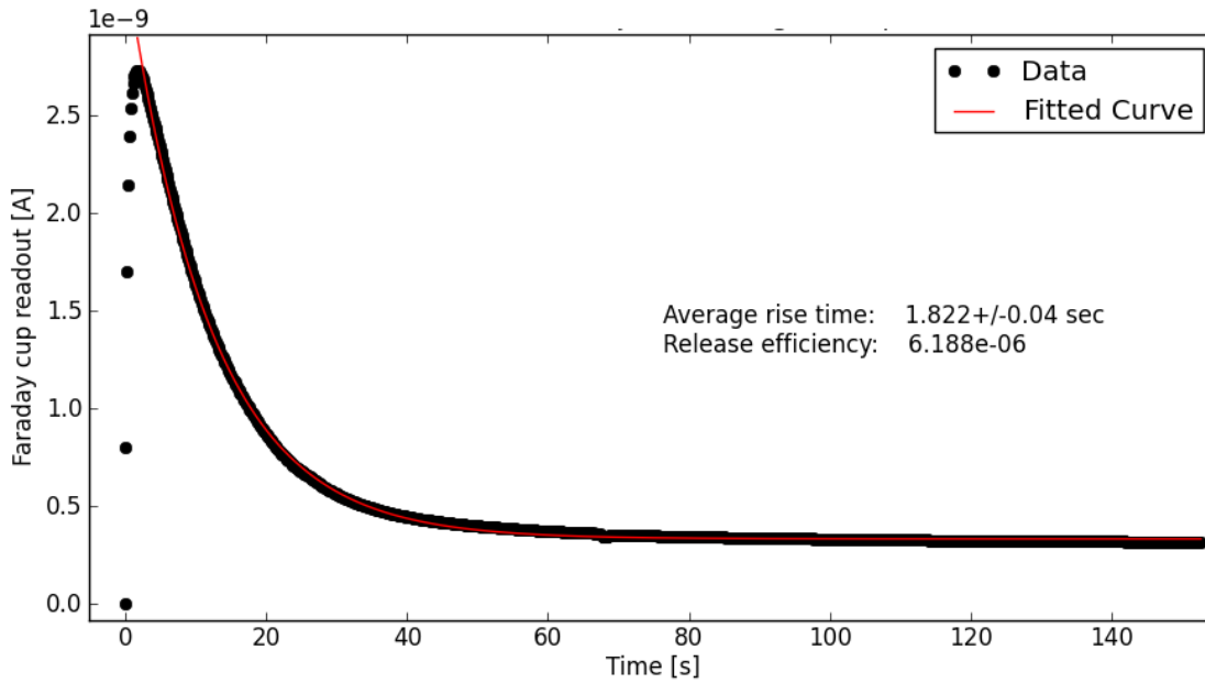
Figure 2.11.: Typical measurement of release of injected gas. In this case the release of ^{13}\text{CO}^+ was monitored after the injection of ^{13}\text{CO}_2 from a plain tantalum target container heated to 1500\text{ }^\circ\text{C} . The presented peak is an average of 82 injections.
