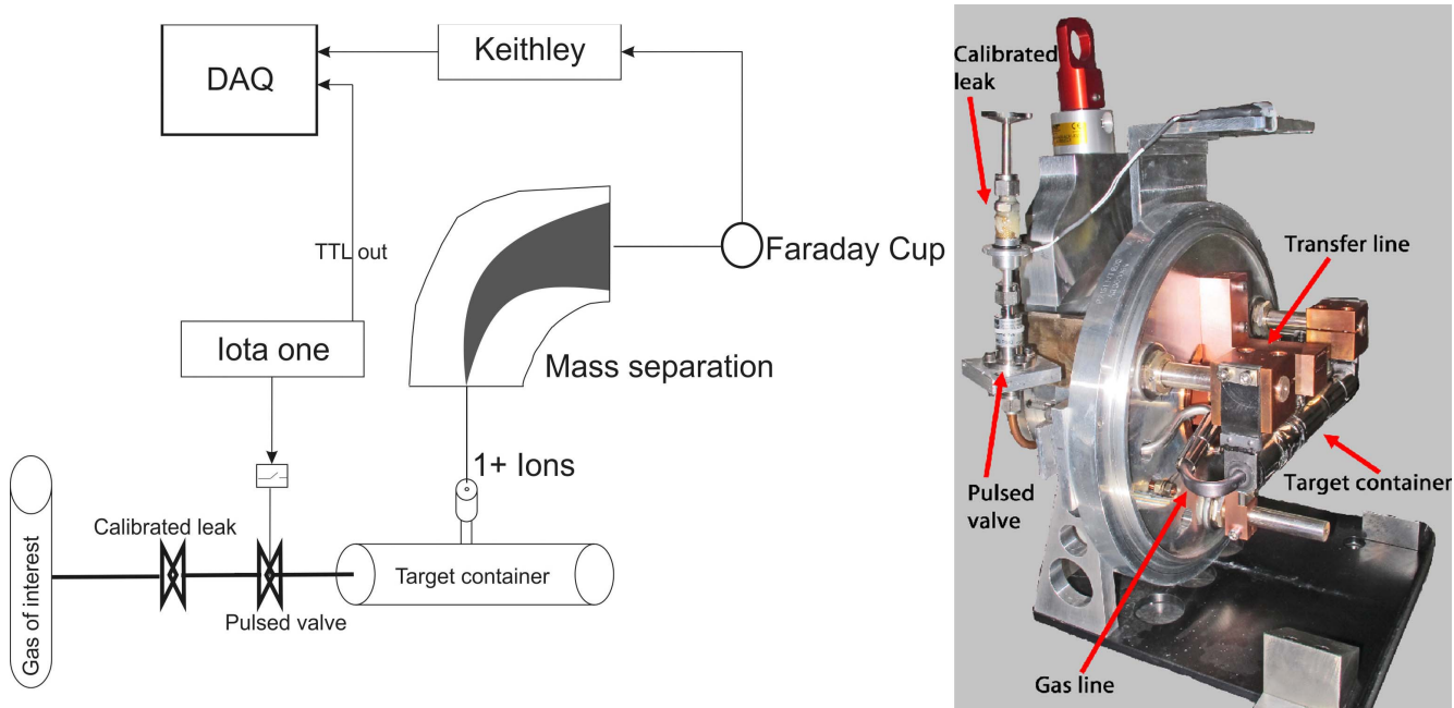
Figure 2.9.: Setup for release measurements. The gas of interest (e.g. CO, CO 2 , Ne, Ar,..) is injected pulse by pulse via a pulsable high speed valve into the target container. Depending on the nature of the injected gas, adsorption or chemical reactions with the container materials can occur during the migration to the ion source. After the extraction, ions are mass separated and the current of +1 ions monitored via a Faraday cup.
