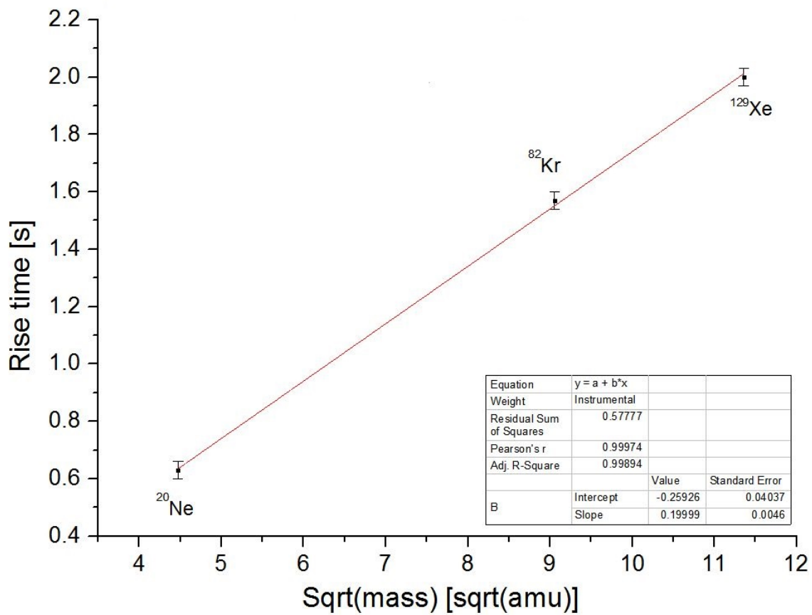
Figure 2.13.: The plot shows the linear correlation of rise time with the square root of the mass as shown in equation 2.9. Measurements were taken with T_{target} = 800^{\circ}C and p_{gas} = 0.4bar .
