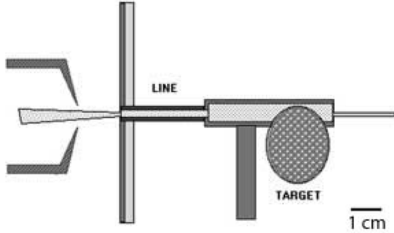
Figure 1.7.: The picture shows a cross section of a target arrangement using a surface ion source. The heated tube is connected in the center of the target container. Protons impinge the target container perpendicular to the drawing plane.
