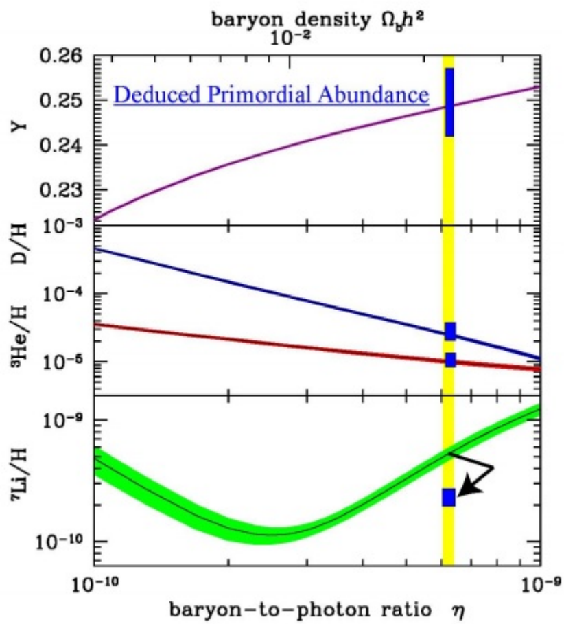
Figure 3.19.: Relative abundances of D, {}^3\text{He} , {}^4\text{He} ( Y ) and {}^7\text{Li} to {}^1\text{H} in dependency of the Baryon to photon ratio \eta . In the case of {}^7\text{Li} the green line indicates the expected abundance while the blue square marks the observed. Picture taken from [92]
