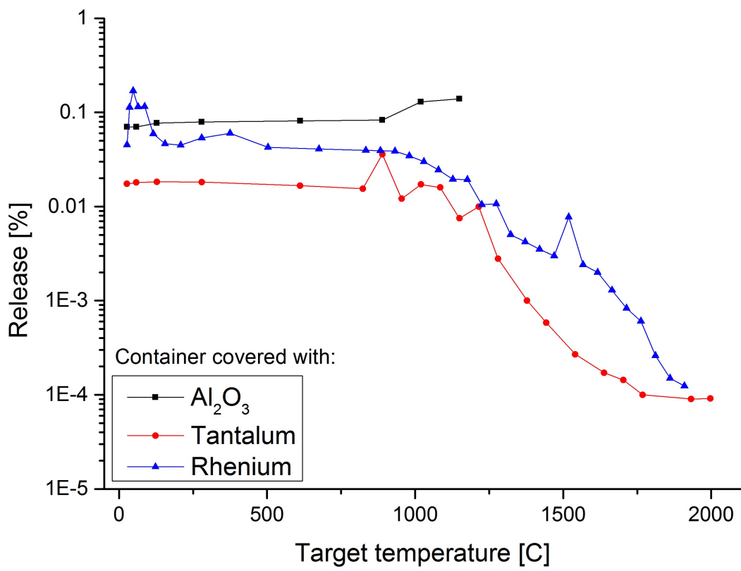
Figure 2.14.: Fraction of ^{13}\text{CO}_2 , released as ^{13}\text{CO}_2^+
