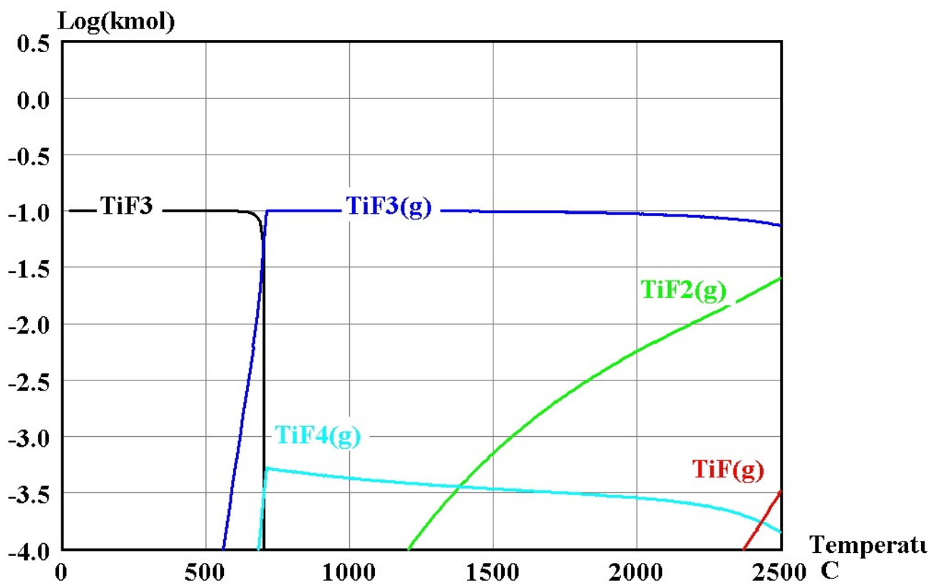
Figure 4.2.: Chemical equilibrium of Titanium with carbon tetrafluoride CF_4 in presence of tantalum.
