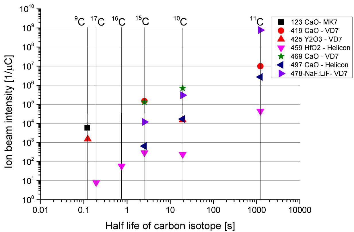
Figure 2.20.: Obtained yields of carbon isotopes extracted as CO^+ during online runs from different target units. The legend indicates the target unit number, the used target material and ion source.
