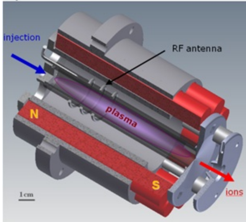
Figure 1.11.: Helicon ion source from [33]
