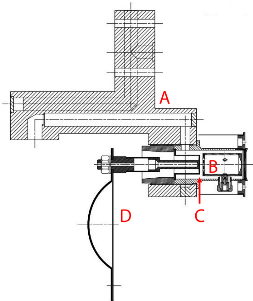
Figure 2.17.: Sketch of the VADIS ion source with a cold transfer line. A: Copper transfer line, B: Anode, C: Cathode, D: Connection for resistive heating.
