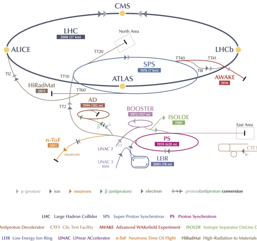
Figure 1.3.: ISOLDE in the CERN accelerator complex. The Protons for ISOLDE are accelerated by the LINAC 2 and the Booster up to 1.4 GeV.
