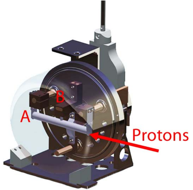
Figure 1.5.: One possible set-up of an ISOLDE target unit. To see here with a standard target container (A), a cold copper transfer line (B) and a Febiad ion source (C).
