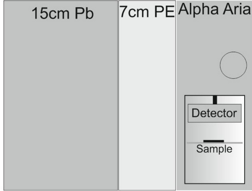
Figure 3.6.: Set up for detection of alpha particles coming from the ^{10}\text{B}(n, \alpha)^7\text{Li} reaction. In order to moderate the neutrons coming from the Pu-Be source, 7 cm of PE are placed in front of the Ortec Alpha Aria detector. Additional 15cm of lead help reducing the background in the measurement.
