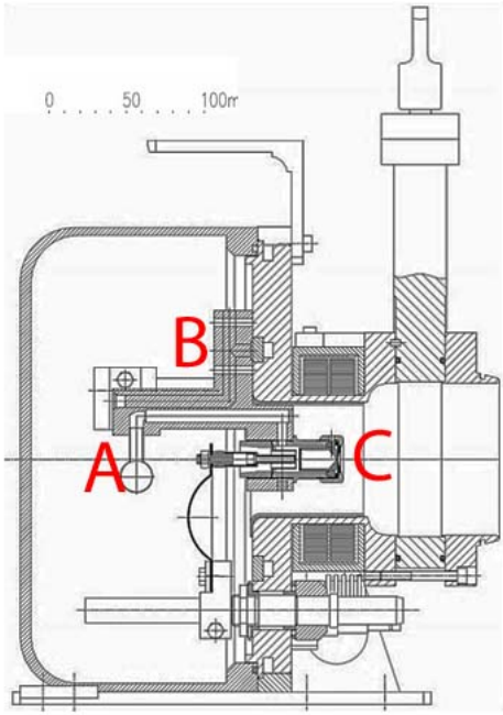
Figure 1.5.: One possible set-up of an ISOLDE target unit. To see here with a standard target container (A), a cold copper transfer line (B) and a Febiad ion source (C).
