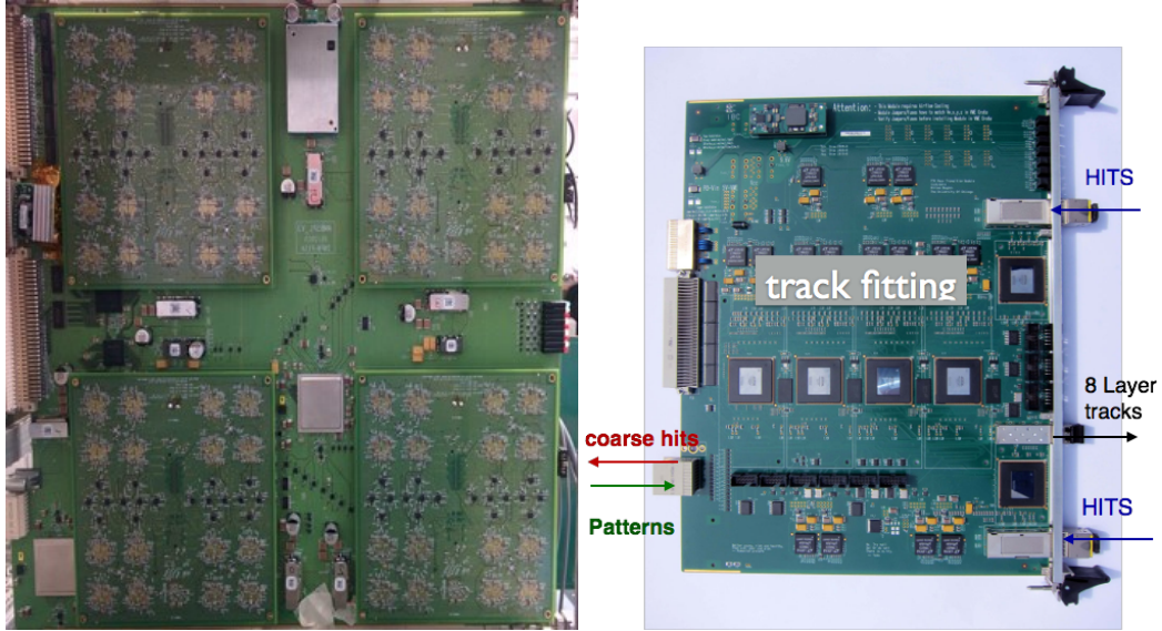
Figure 2. The two pictures show a fully loaded AMBSLP board, with 4 LAMB cards installed for a total of 64 AM chips. Although the AM chips are not visible as they are mounted on the card, the socket footprint is clearly visible. The right picture shows an AUX card with the 4 Altera Arria V FPGAs, which are used for the linear fit.
