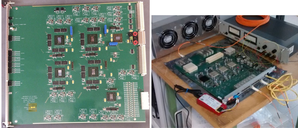
Figure 3. The left picture shows a recent prototype of the SSB. In the center of the board, the 4 FPGAs devoted to the final track fit are clearly visible. The right picture shows a FLIC board.
