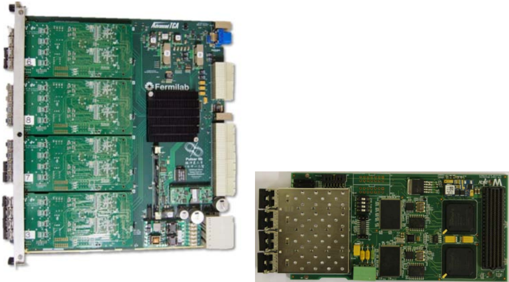
Figure 1. The pictures show a fully stuffed DF board (left), with 4 FTK_IM installed. The right picture shows a detailed view of the a FTK_IM prototype, with the two FPGAs close to the FMC connector. The DF is able to receive 16 fibers.
