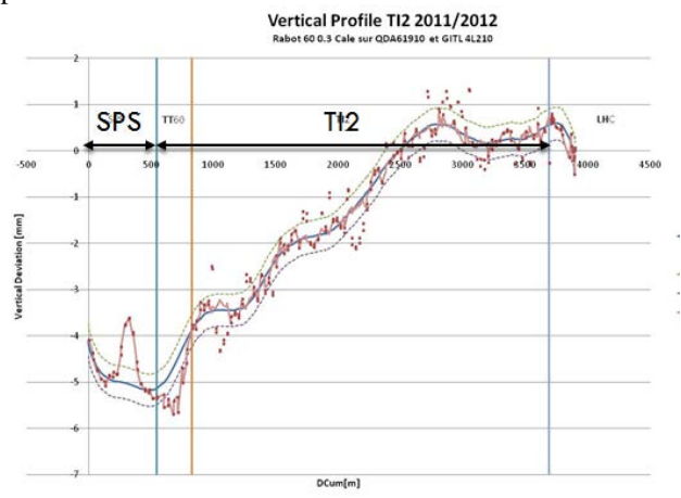
Figure 3 : vertical deviation of TI2 quadrupoles magnets
