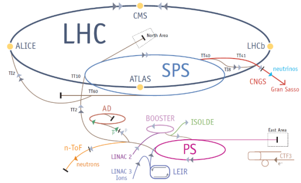
Figure 1 : the LHC and the Injectors complex
