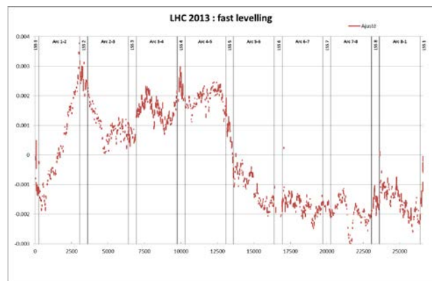
Figure 8 : the LHC vertical profile
