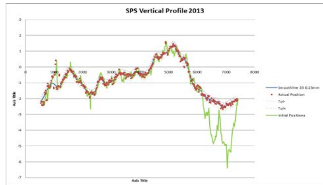
Figure 7 : the SPS vertical profile after realignment
