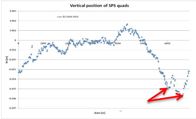
Figure 2 : vertical deviation of SPS quadrupoles magnets
