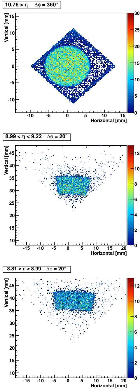
Figure 5.13: The true incident position distributions for the events in which hit position was reconstructed in each fiducial area obtained by using the EPOS 1.99 model. Horizontal and vertical axes represent the transverse distance from the beam center position.
