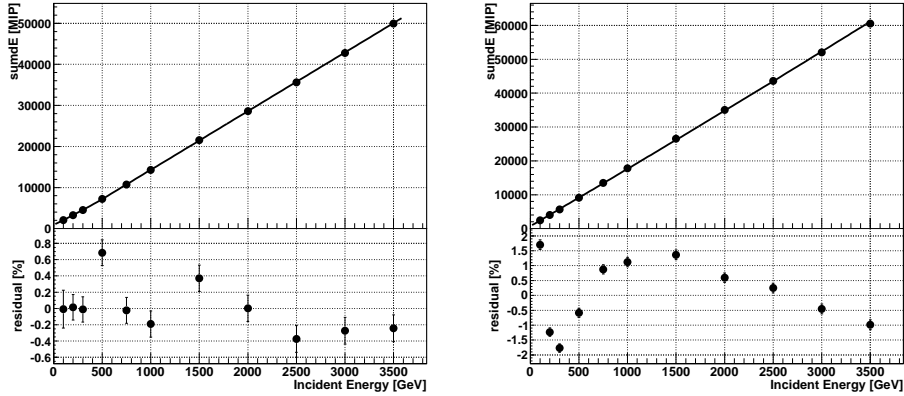
Figure 3.7: The energy response function for the Arm1 detector obtained by MC simulation with QGSJET II-03. The left and the right figures correspond to the small tower and the large tower, respectively. The upper panels show the relations between the incident energy and the average of sumdE. The black curves are the results of fitting. The bottom panels show the residuals from the fitting.
