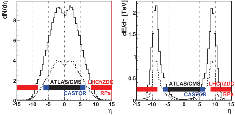
Figure 2.4: Particle distribution as a function of pseudo-rapidity \eta . Left shows the multiplicity and right shows energy flux for charged+neutral particles (solid) and neutral particles (dashed).
