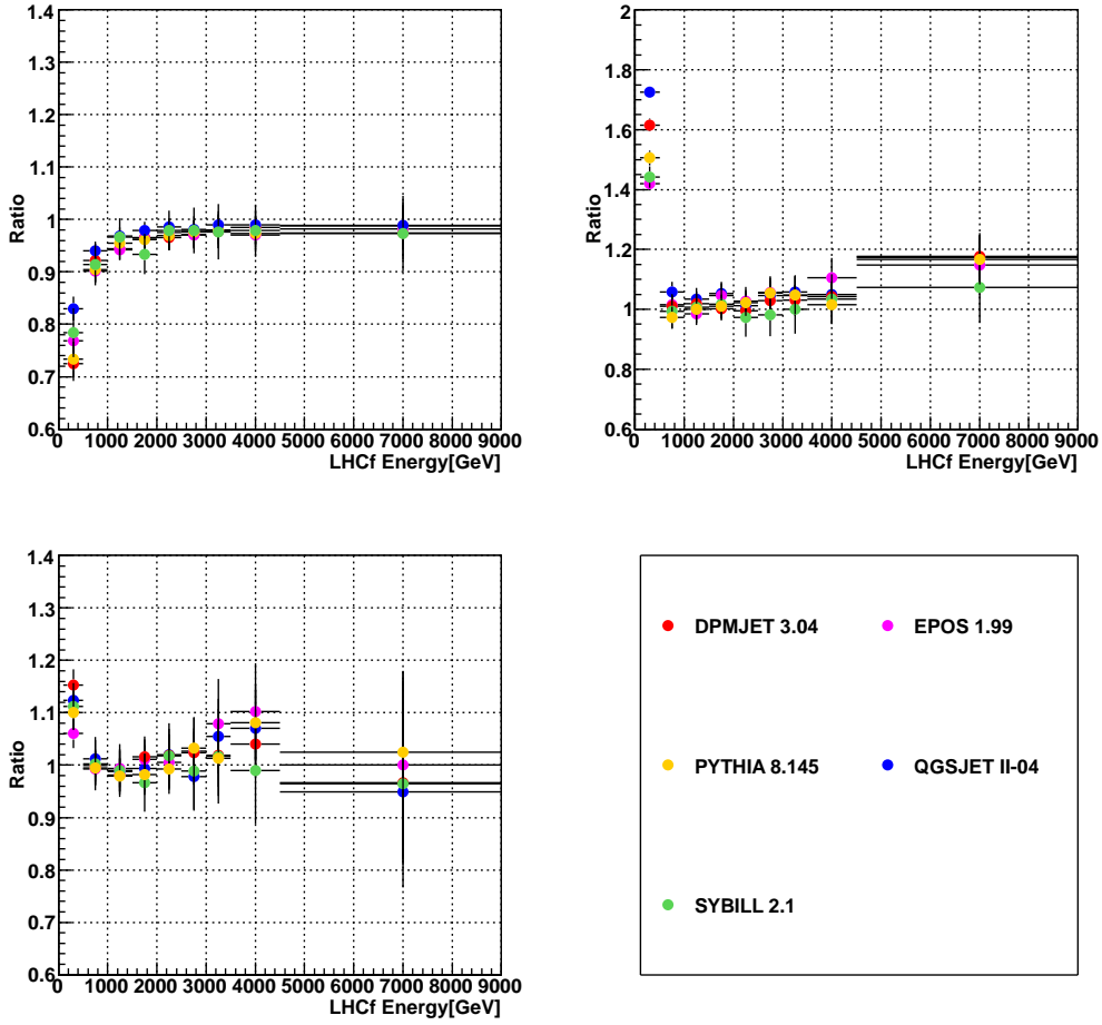
Figure 5.15: The ratio between the ( E_{posrec} ) and the ( E_{postrue} ) estimated by each hadronic interaction model. The upper left, the upper right, and the bottom panels correspond to the small tower, the large tower A, and large tower B, respectively.
