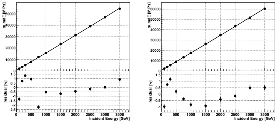
Figure 3.8: The energy response function for the Arm2 detector obtained by MC simulation with QGSJET II-03. The left and the right figures correspond to the small tower and the large tower, respectively. The upper panels show the relations between the incident energy and the average of sumdE. The black curves are the results of fitting. The bottom panels show the residuals from the fitting.
