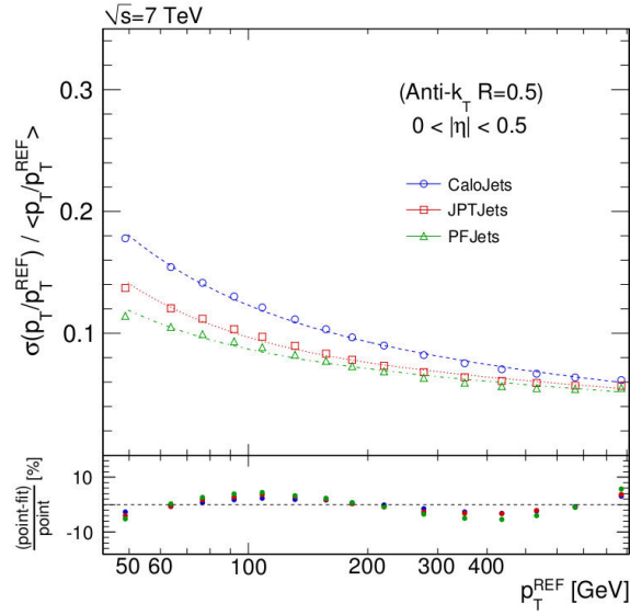
Figure 6.3.: Illustration of the jet p_T resolution from MC truth as a function of p_T^{\text{ref}} , taken from [132]. The jet resolution is shown for Calo-, JPT- and PFJets in the very central detector region with |\eta| < 0.5 .
