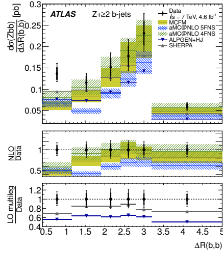
Figure 8: The differential cross-section for Z+\geq 2b -jets as a function of the opening angle \Delta R(b, b) [10].
