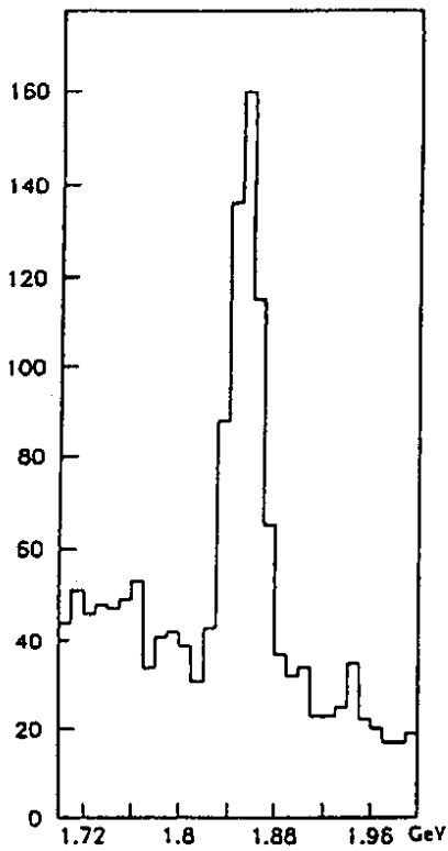
(a) D^0 \rightarrow K^- \pi^+ ( N_\sigma > 4 );
