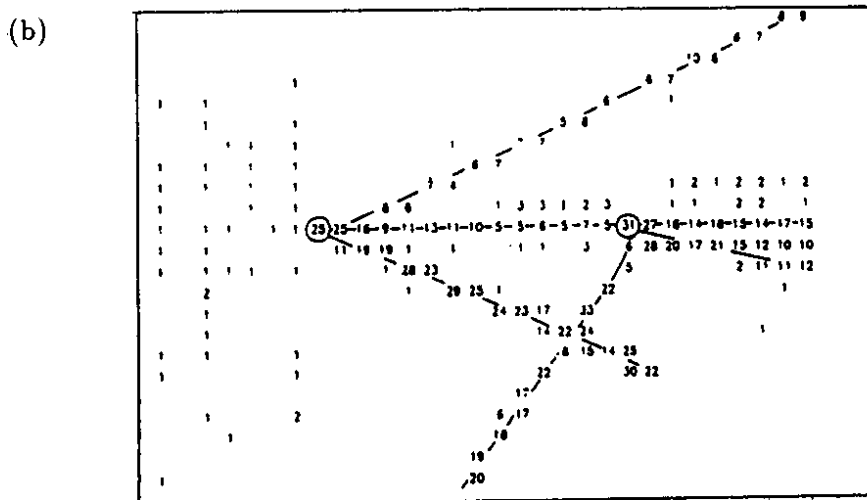
Fig. 6. (a) An event with both charmed particles reconstructed; (b) A secondary interaction.
