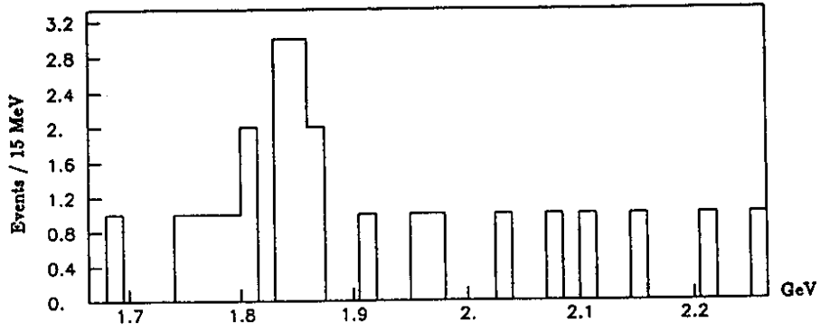
Fig. 10. D^0 \rightarrow \phi \pi^+ \pi^- mass distribution ( N_\sigma > 6 ).
