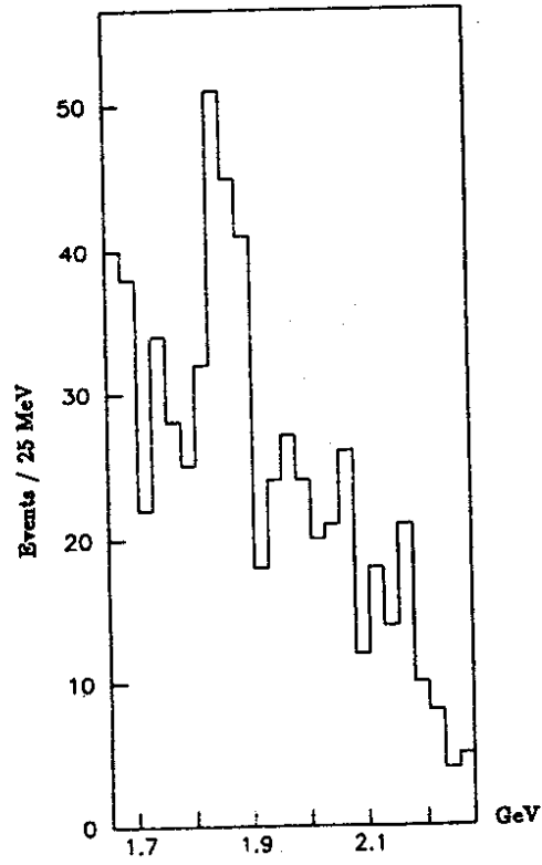
Fig. 8. D^0 \rightarrow K^- \pi^+ \pi^0 mass distribution ( N_\sigma > 8 ).
