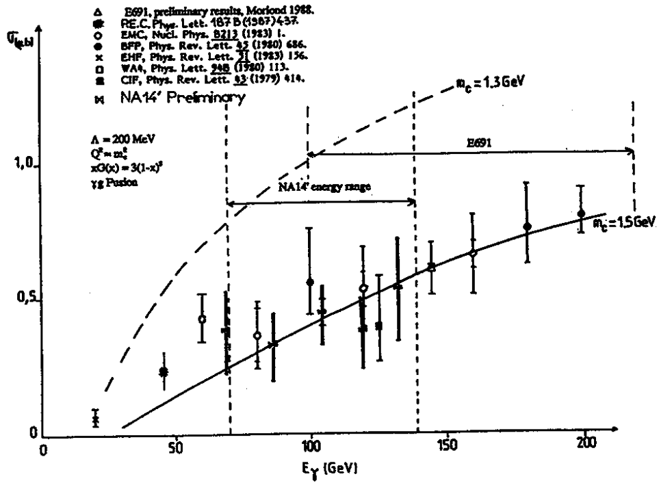
Fig. 23. Energy dependence of the charm photoproduction cross-section.
