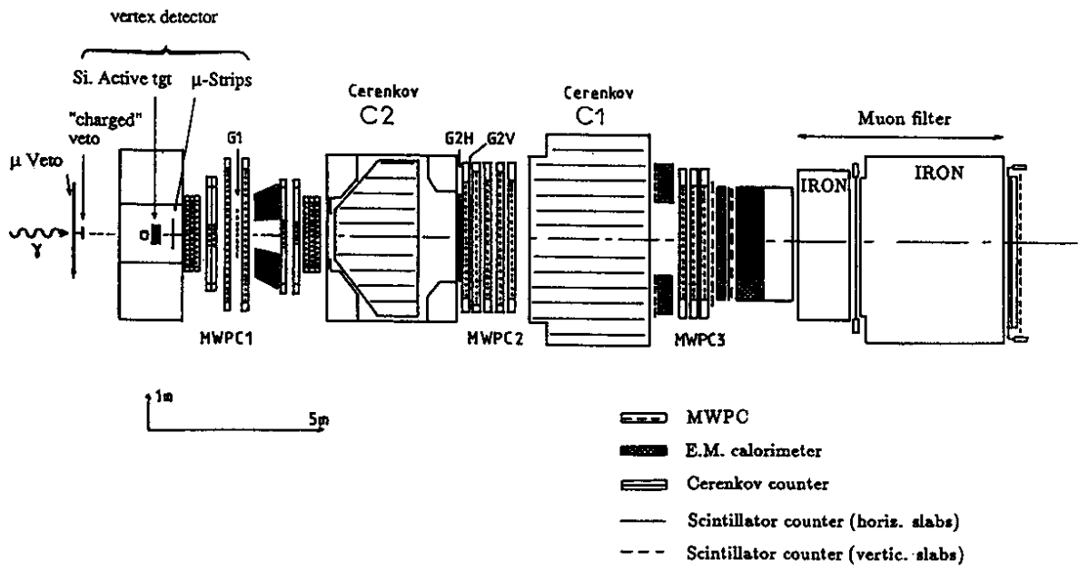
Fig. 1. The NA14' spectrometer.
