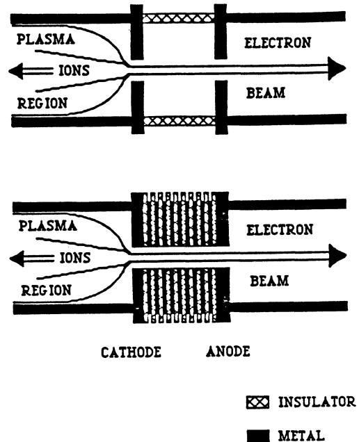
Fig. 1 - Schematic of single-gap (top) and multigap (bottom) pseudo-spark chambers, showing the discharge geometry.
