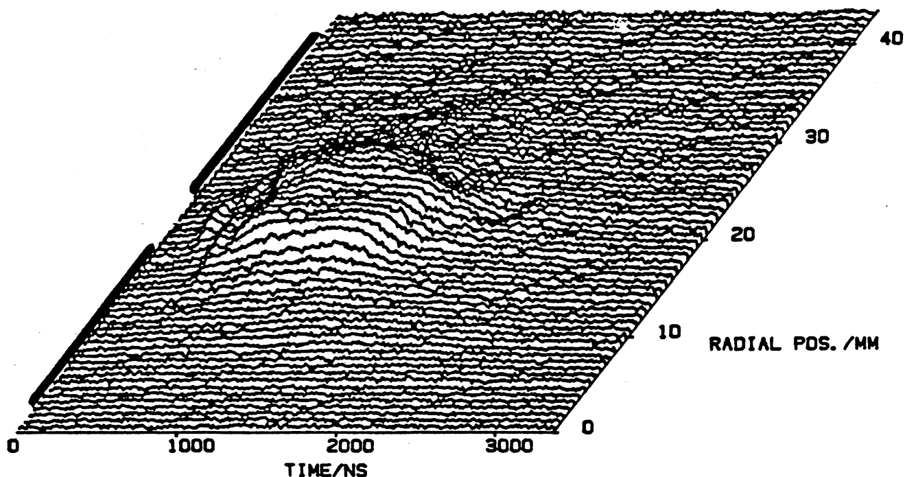
Fig. 6 - The streak photograph of a flash bulb triggered BLT plasma shows the homogeneous dense glow in the centre of the electrodes, and a very faint glow outside, decreasing to almost zero intensity at the electrode edges. The picture was taken as a single shot recording at a wavelength of 486.1 nm ( H\beta ), at a voltage of 10 kV/4 kA and a hydrogen filling pressure of 20 Pa. The FWHM of the slightly underdamped current pulse is approximately 1 \mu s.
