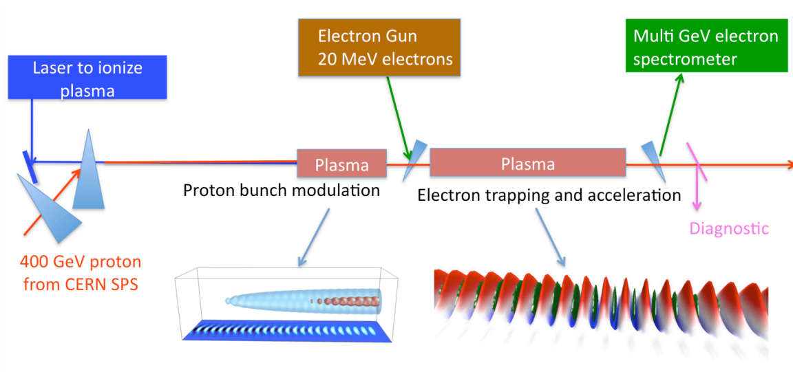
Figure 3. Conceptual design of the AWAKE experiment, showing the major sections and description of expected effects.
