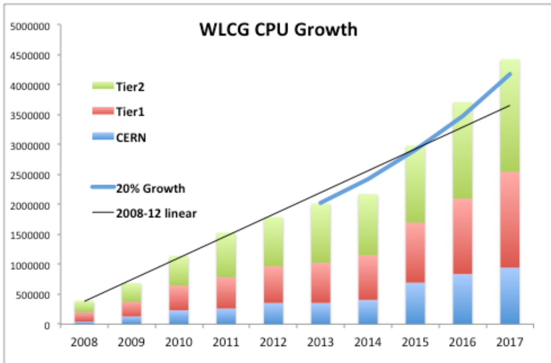
Figure 12: Summary of total CPU requirements
