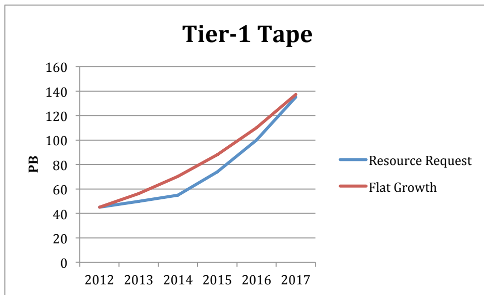
Figure 41: Evolution of CMS Tier 1 Tape
