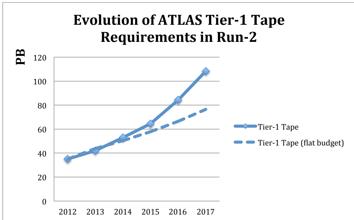
Figure 33: Evolution of ATLAS Tier 1 Tape
