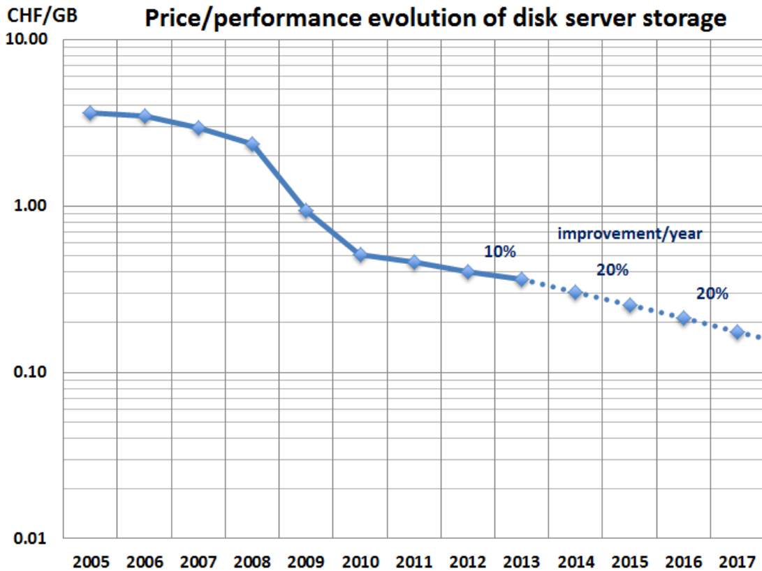
Figure 25: Evolution of price/performance of disk, example of CERN computer centre
