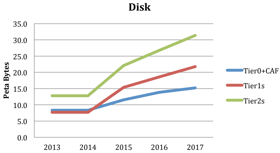
Figure 30: Disk requirement profile. Disks can be installed any time during a given year or during the previous year
