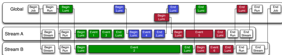
Figure 17: Multi-threaded CMSSW design
