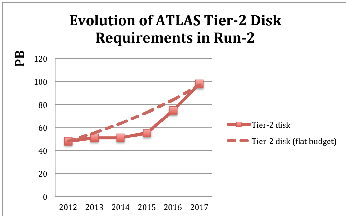
Figure 35: Evolution of ATLAS Tier 2 Disk
