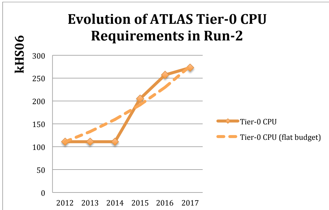
Figure 36: Evolution of ATLAS Tier 0 CPU
