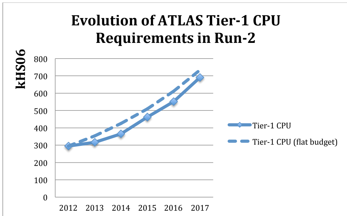
Figure 31: Evolution of ATLAS Tier 1 CPU
