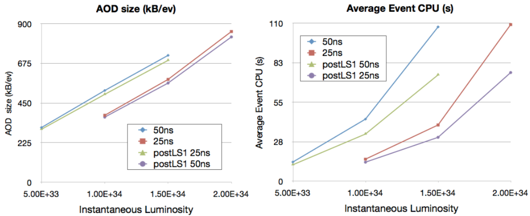
Figure 16: Performance metrics for the latest CMSSW release
