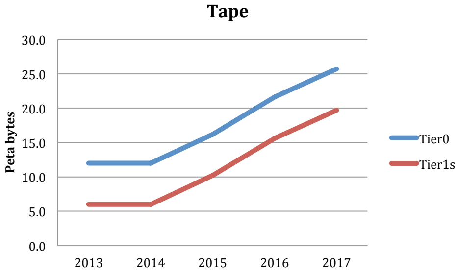
Figure 29: Tape requirement profile. Resources for a given year can be installed at the beginning of the following year.
