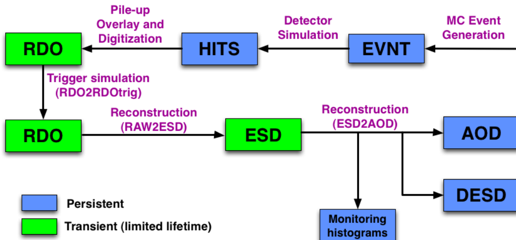
Figure 5: ATLAS Monte Carlo Simulation Data flow
