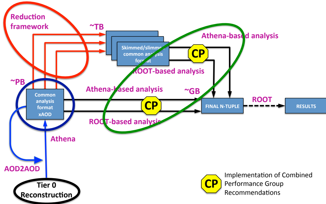
Figure 3: A schematic view of the new ATLAS Analysis Model, highlighting the main areas of software activity required for its implementation. xAOD EDM and implementation - black and blue areas; xAOD reduction framework - red area; analysis releases and dual use tools - green area
