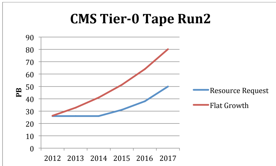
Figure 46: Evolution of CMS Tier 0 Tape
