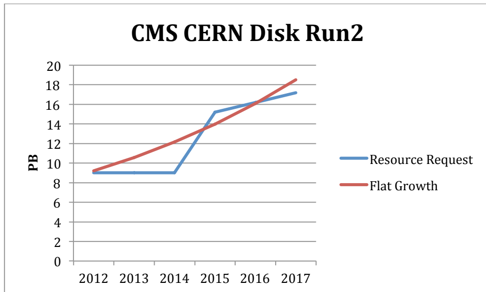
Figure 45: Evolution of CMS Tier 0 Disk
