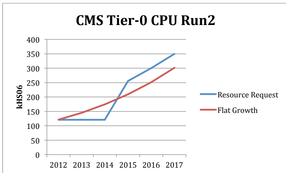
Figure 44: Evolution of CMS Tier 0 CPU
