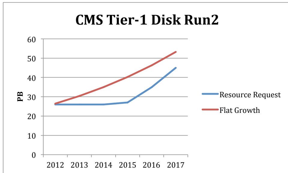
Figure 40: Evolution of CMS Tier 1 Disk
