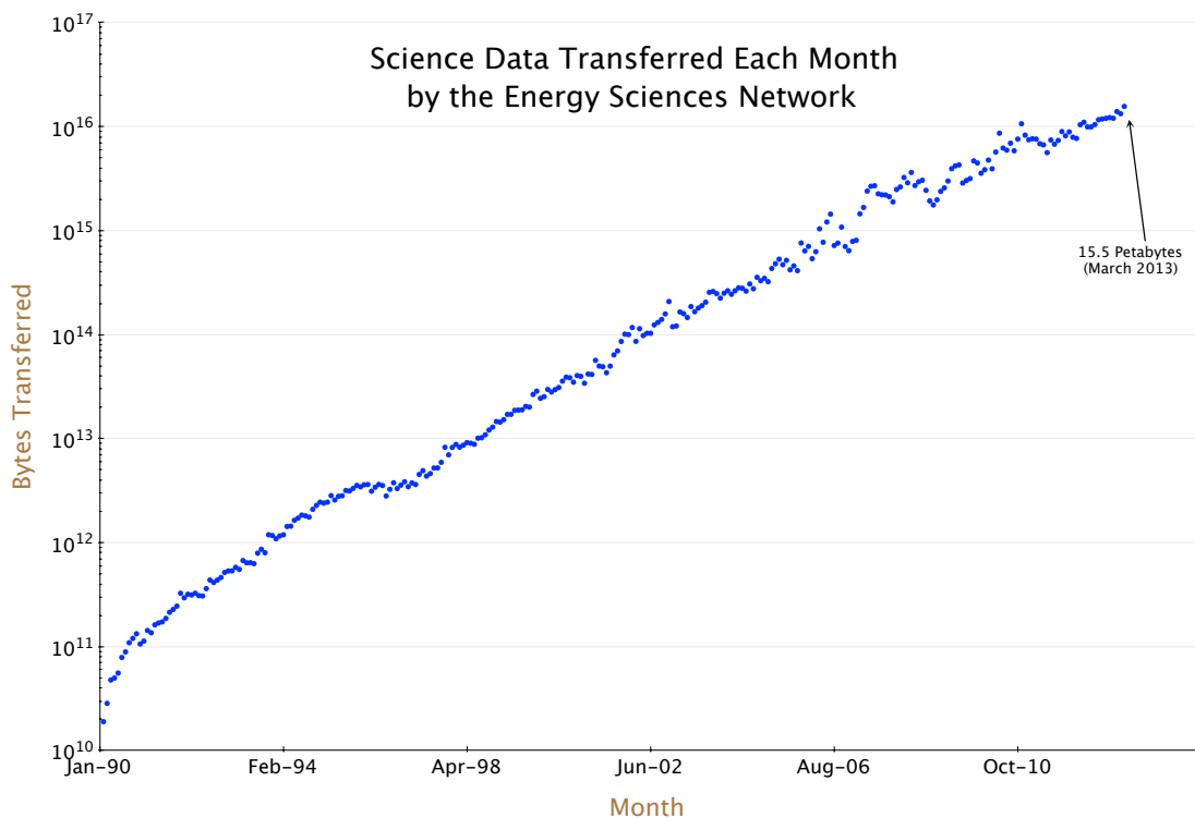
Figure 20: Network traffic transferred by DOE’s Energy Sciences Network, in bytes per month, since 1990. Traffic doubles every 18 months.
