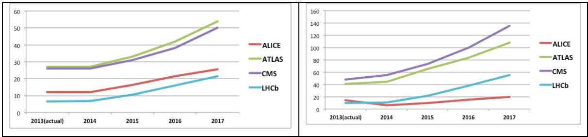
Figure 11: Tape summary; Tier 0 (left), Tier 1 (right)
