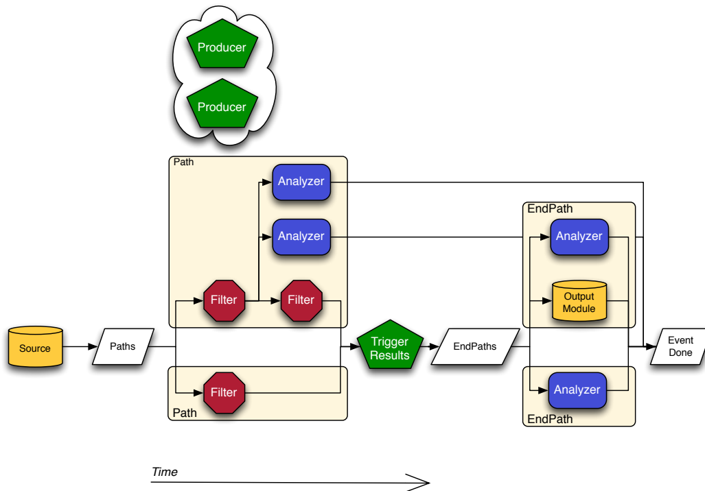
Figure 18: Illustration of sub-event parallelism
