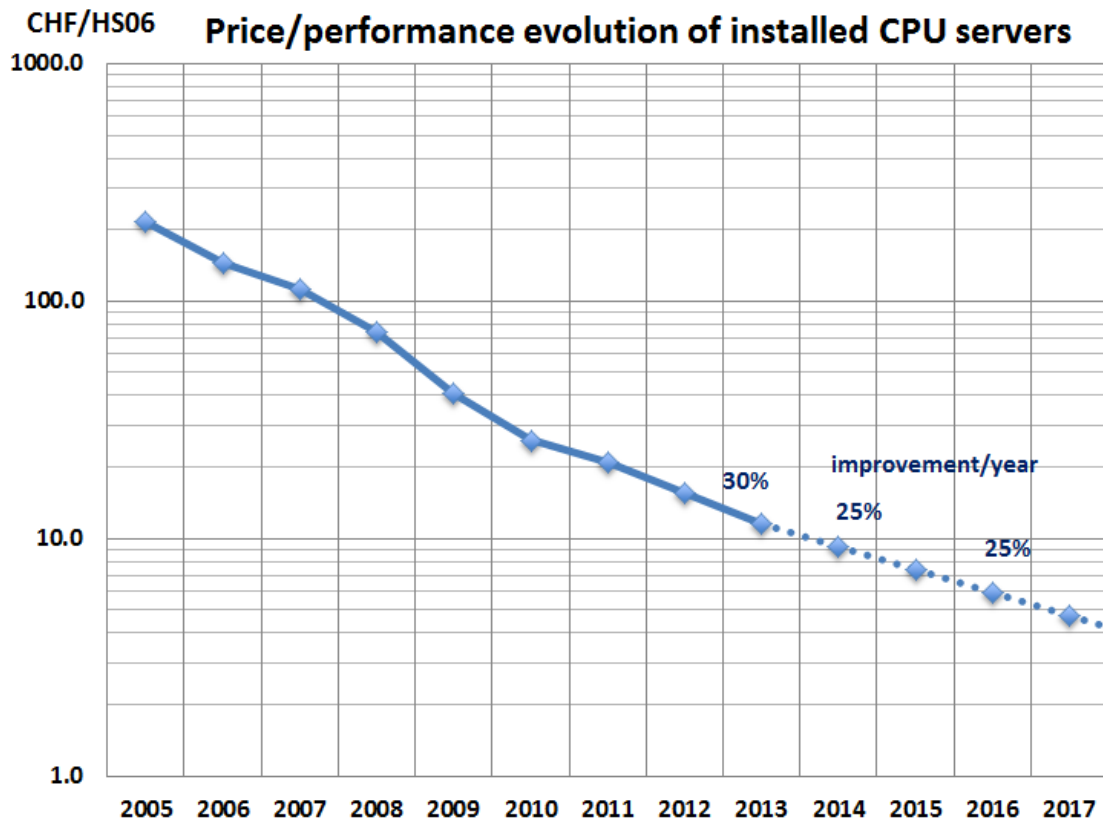
Figure 22: Evolution of price/performance of server systems, example of the CERN computer centre
