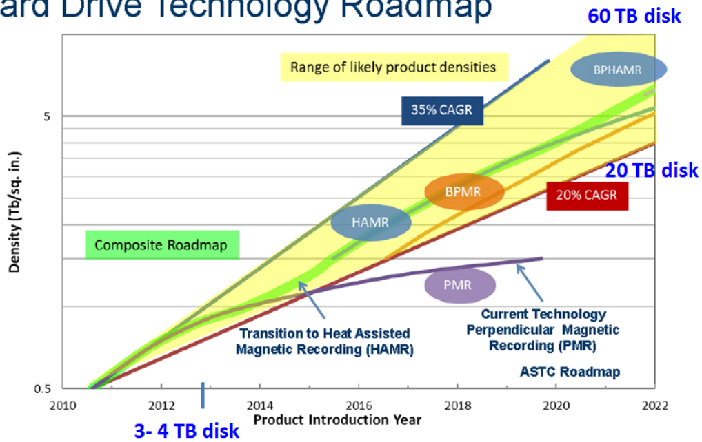
Figure 24: Disk technology roadmap
