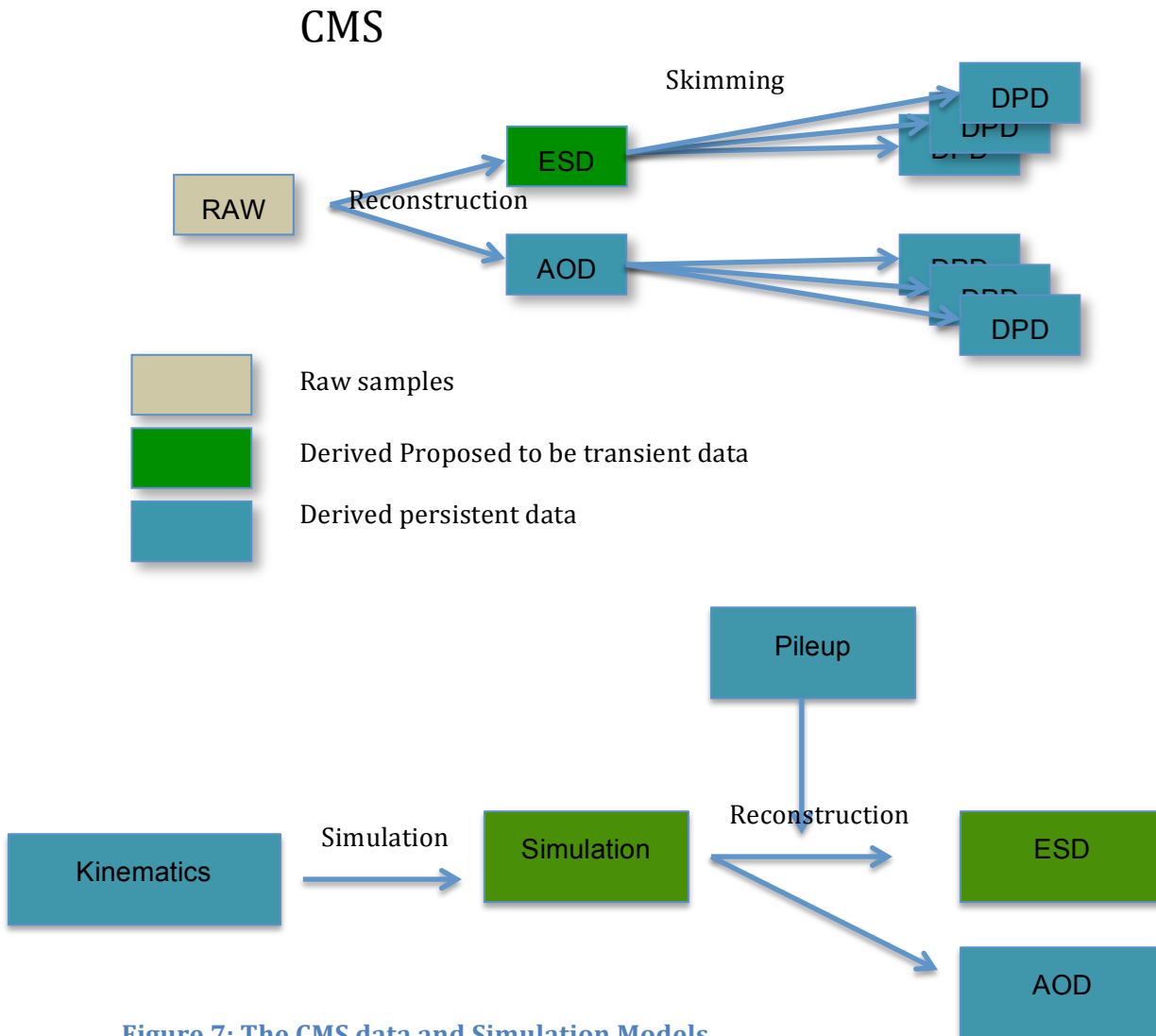
Figure 7: The CMS data and Simulation Models
