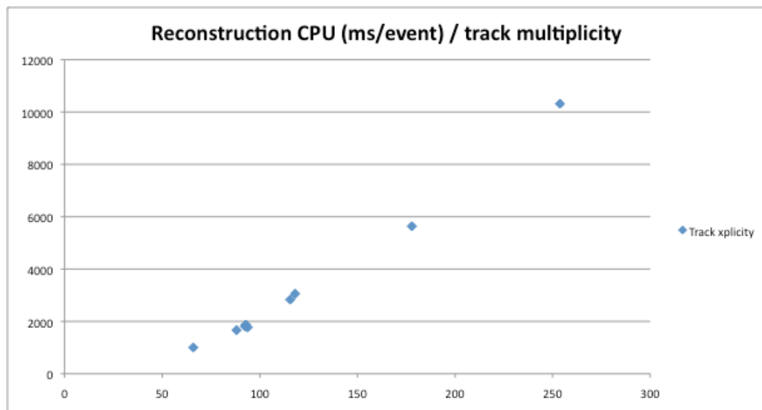
Figure 19: LHCb reconstruction time vs track multiplicity
