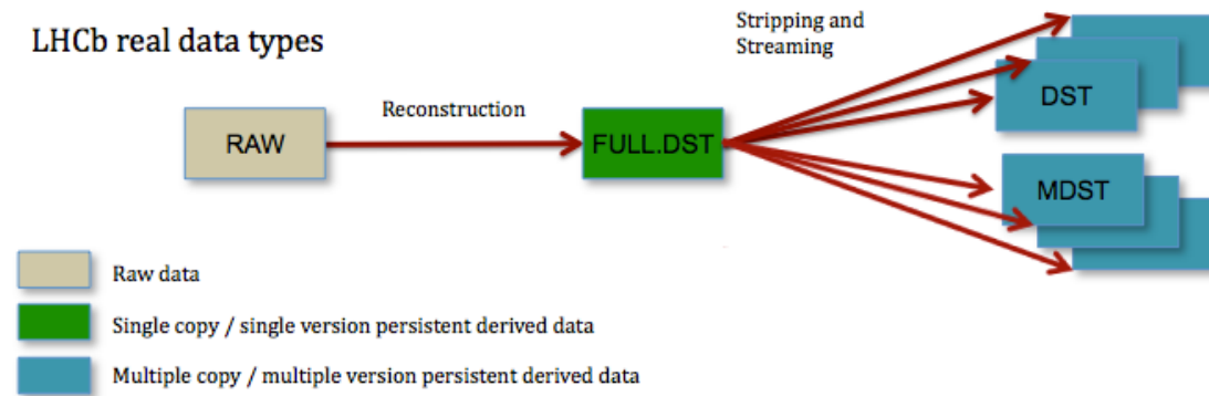
Figure 8: The LHCb Data model
