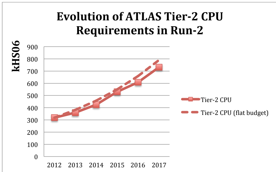
Figure 34: Evolution of ATLAS Tier 2 CPU
