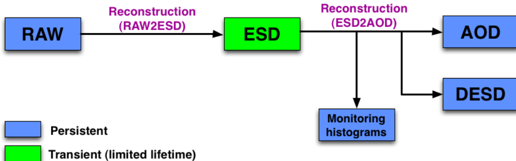
Figure 4: ATLAS Reconstruction Data Flow
