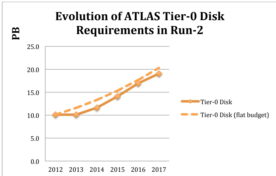
Figure 37: Evolution of ATLAS Tier 0 Disk
