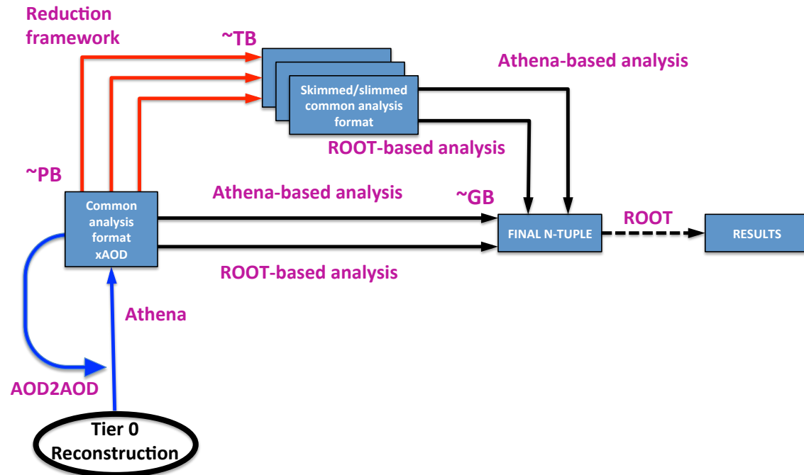
Figure 6: ATLAS Analysis Data Flow
