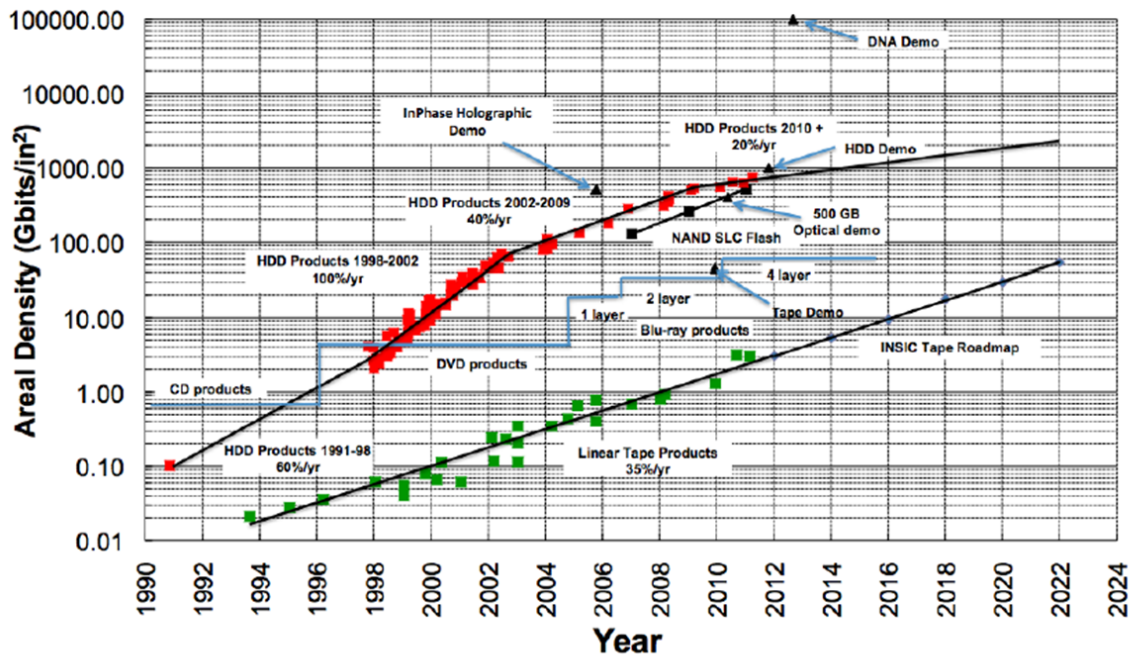
Figure 23: Storage technology areal density trends
