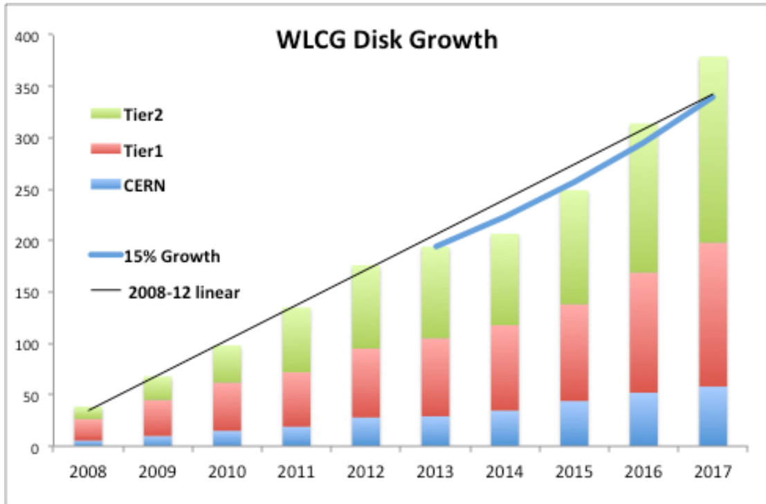
Figure 13: Summary of total disk requirements
