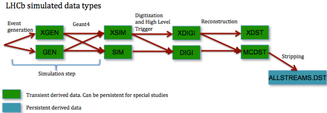
Figure 9: LHCb simulated data processing
