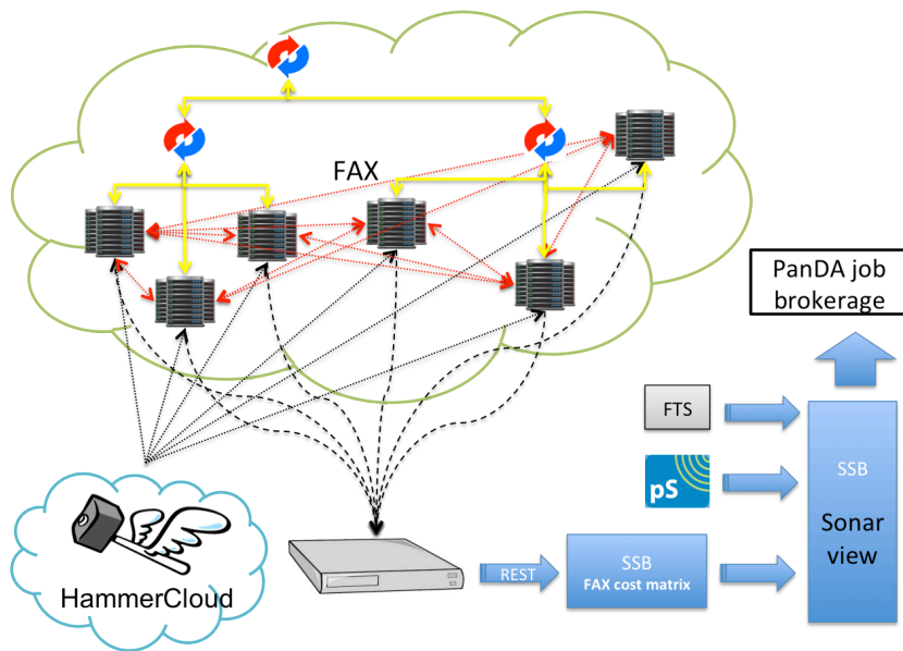
Figure 5. Measuring rates between job queues and FAX endpoints. Jobs submitted by HammerCloud tasks measure the interlinks and report values to the SSB. Information is filtered and averaged before sending to PanDA (standalone or in combination with FTS and perfSonar measurements).
