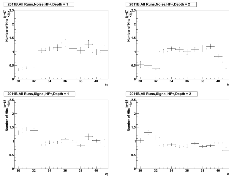
Figure 6.11. Average noise and signal rates for HF+ i\phi = 67 for the 2011B dataset. The top histograms are for noise hits, the histograms on the bottom are for signal hits.
