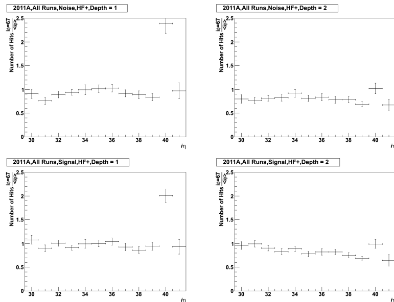
Figure 6.12. Average noise and signal rates for HF+ i\phi = 67 for the 2011A dataset. The top histograms are for noise hits, the histograms on the bottom are for signal hits.
