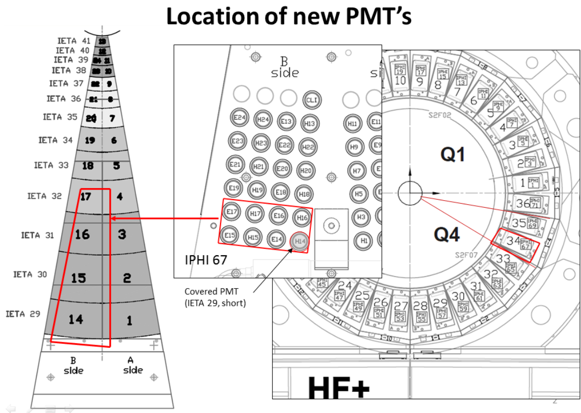
Figure 5.5. Schematics showing the location of the eight PMTs installed in the HF+.
