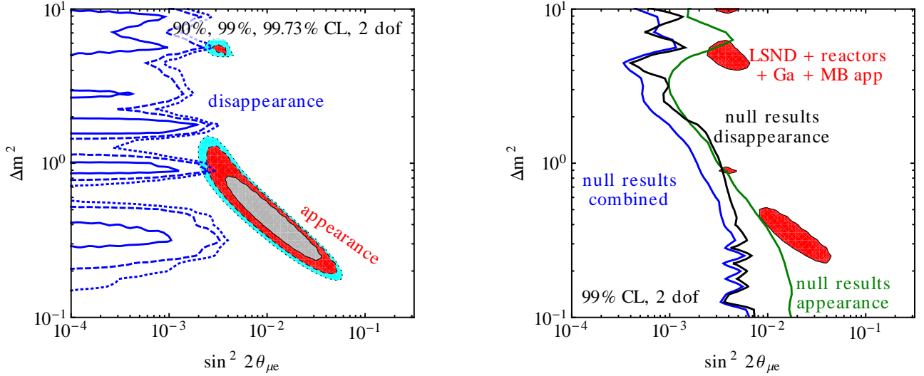
Figure 3: Global constraints on sterile neutrinos in a 3+1 model. In the left panel, we show that \bar{\nu}_e appearance data (coloured region: LSND [7], MiniBooNE [123], KARMEN [129], NOMAD [130], E776 [131], ICARUS [132]) is only marginally consistent with disappearance data (blue contours: atmospheric neutrinos [133], solar neutrinos [134–143], MiniBooNE/SciBooNE [164, 165] MINOS [144, 145], reactor experiments [3, 166–176], CDHS [146], KARMEN [177] and LSND [178] \nu_e - ^{12}\text{C} scattering data and gallium experiments [14, 16, 17, 135]). In the right panel, we have split the data into those experiments which see unexplained signals (LSND, MiniBooNE appearance measurements, reactor experiments, gallium experiments) and those which don’t. For the analysis of reactor data, we have used the new reactor flux predictions from [10], but we have checked that the results, especially regarding consistency with LSND and MiniBooNE \bar{\nu} data, are qualitatively unchanged when the old reactor fluxes are used. Fits have been carried out in the GLoBES framework [179, 180] using external modules discussed in [152, 162, 181, 182].
