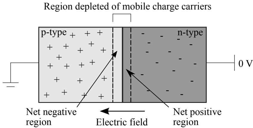
(b) Unbiased p-n junction after thermal diffusion of mobile charged carriers.
