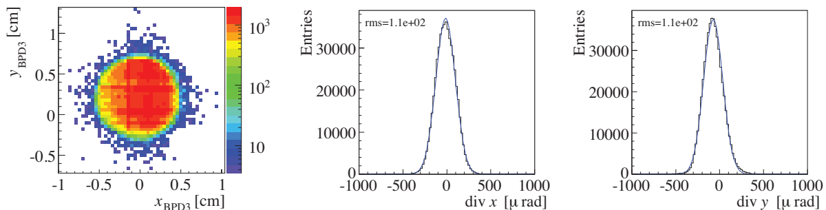
Figure 5.2: The beam spot as measured by BPD3 (left) and the x - and y -divergence (middle and right) of the 2007 beam. Distributions are based on all thin target runs of the 07L production, where BPD-Cut (I) and (II) have been applied (see Section 6.3).
