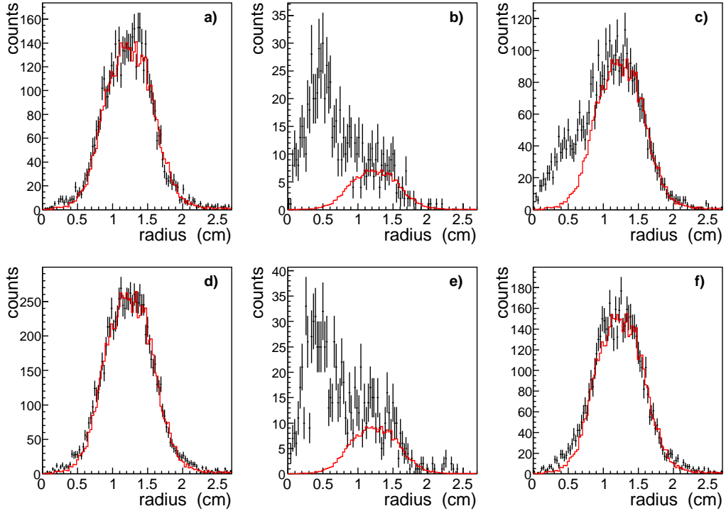
Figure 5: Radial annihilation distributions for the antiproton annihilation vertices for the ETP (a) and (d), HM (b) and (e) and CM (c) and (f) data sets separated into events for which the axial positions are |z| < 0.5 cm ((a)-(c)) and 0.5 < |z| < 1.5 cm ((d)-(f)). Shown in red is the Monte Carlo simulation (see text for details) for antiproton annihilation on the electrode wall fitted in each case to the higher radius (beyond r = 1.25 cm) portion of the data.
