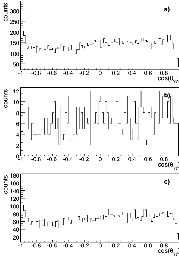
Figure 3: Opening angle plots for the (a) ETP, (b) HM and (c) CM data sets. Only the data for which r > 1 cm (see text) have been selected here to reduce the contribution from protonium annihilations, which tend to be near-axis.
