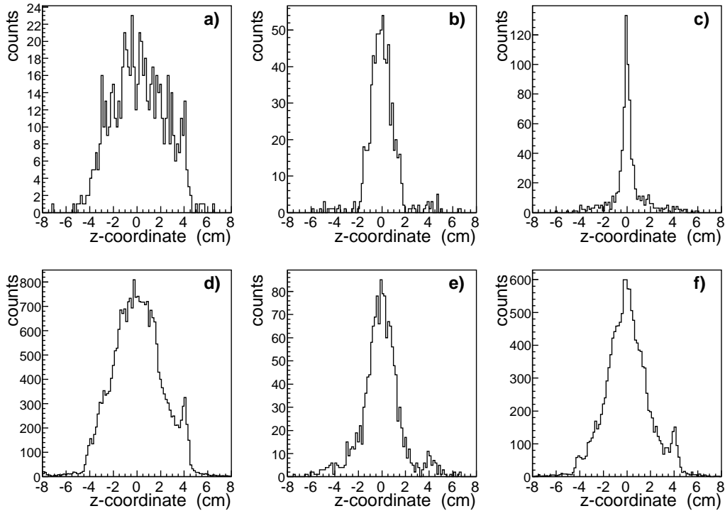
Figure 6: Vertex axial distributions for ETP (a) and (d), HM (b) and (e) and CM (c) and (f) data sets. Boxes (a)-(c) correspond to data for which r < 0.5 cm, with (d)-(f) for r > 0.5 cm.
