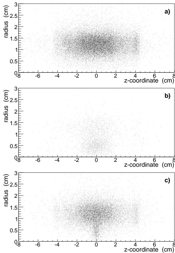
Figure 4: Scatter plots in the r - z plane for the annihilation vertices for the (a) ETP, (b) HM and (c) CM data sets.
