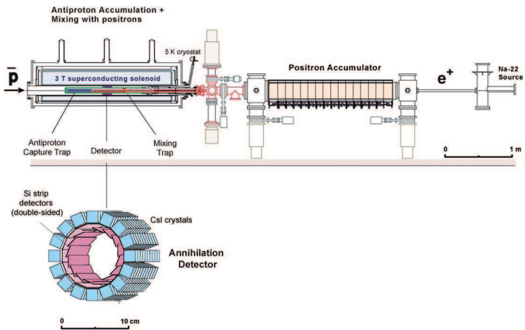
Figure 1: Overview of the ATHENA apparatus showing the positron accumulator, the antiproton trap and the mixing region used to create antihydrogen and protonium. A detector capable of registering both \bar{p} and e^+ annihilations was located around the mixing region and is shown in sketch below the main apparatus [27].
