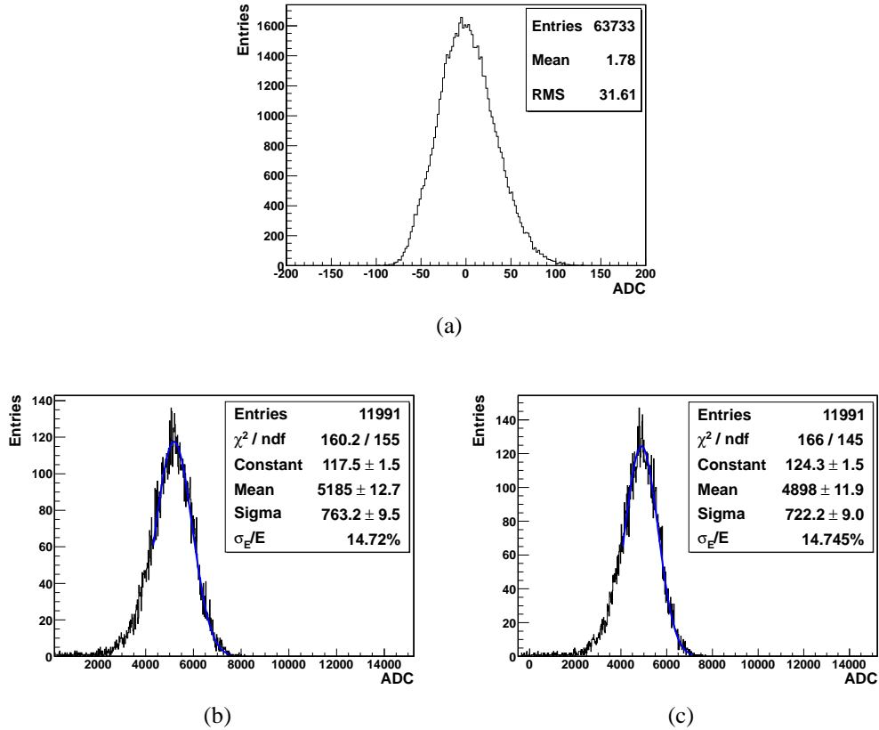
Figure 5.40: Common mode distribution (a) and total energy distribution at 1 GeV with (b) and without (c) the common mode subtraction with a MAROC gain of 10.
