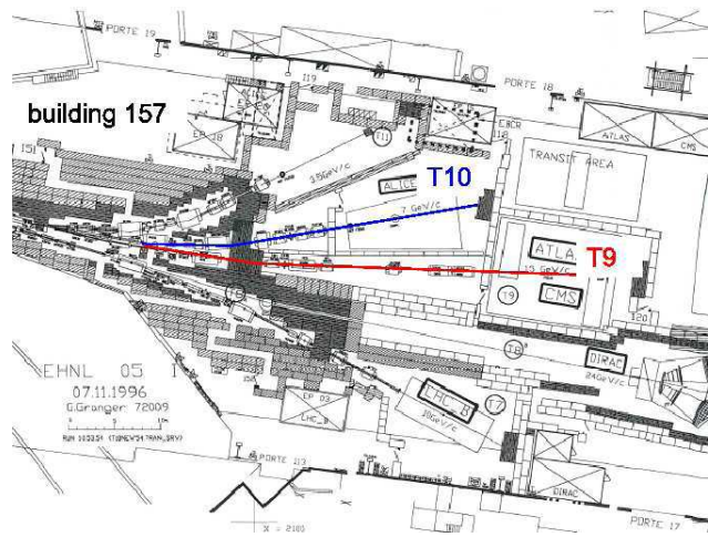
Figure 3.1: The East Hall of the PS complex: the T9 and T10 beamlines are highlighted.
