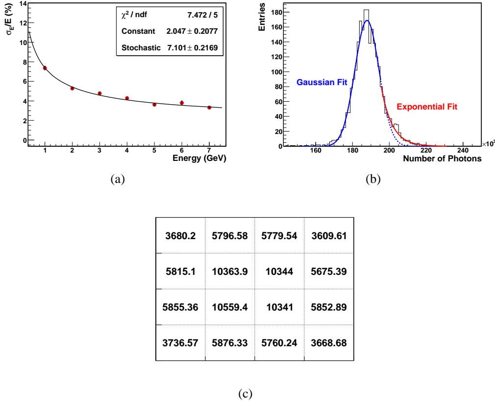
Figure 5.24: Energy resolution (a), photon peak fit without the noise tail (b) and mean number of photons per SiPM (c) using a reflection coefficient of 0.9 and a mirroring efficiency of 0.8.
