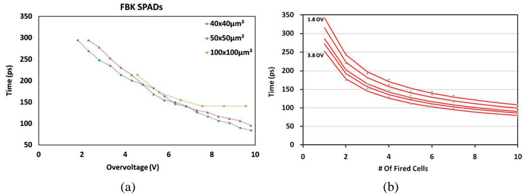
Figure 2.38: Timing resolution as a function of the overvoltage obtained for SPADs with different cell sizes (a) and for 50x50 \mu\text{m}^2 cells SiPMs (b) [70].
