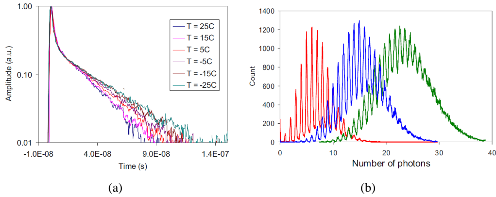
Figure 2.35: Signal shape (a) and pulse height distribution (b) under illumination with variable light pulses of a 1 \text{ mm}^2 area, 400 50 \times 50 \text{ }\mu\text{m}^2 cells FBK-irst SiPM [69].
