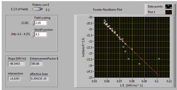
Figure 2: Fowler-Nordheim plot of the field emission in the SRF gun cavity.
