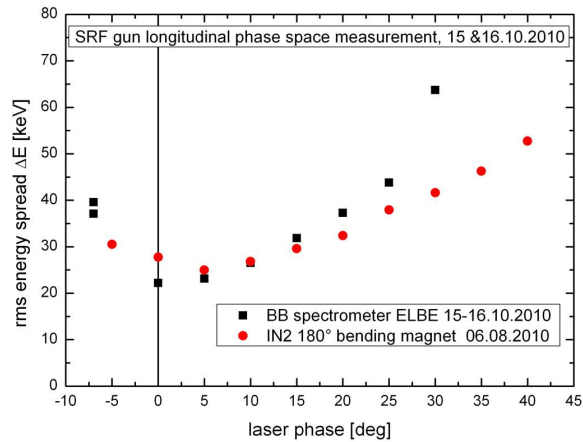
Figure 4: measured curves of the rms energy spread versus the gun phase. The red dots give out the measurement results from the gun diagnostic beam line and the black squares show the result with BB spectrometer in the ELBE beam line.
