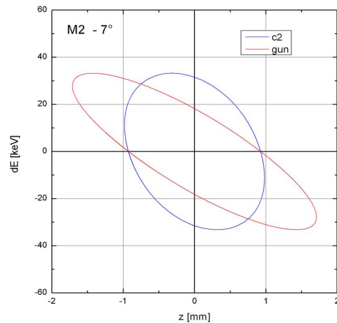
Figure 6: an example of the longitudinal phase space at the exit of the gun cavity with laser phase -7^\circ (red).
