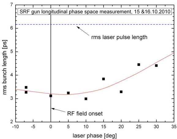
Figure 5: rms bunch length versus the gun laser phase. The blue dotted line shows the rms laser pulse length 6.2ps.
