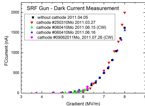
Figure 1: Dark current versus acceleration gradient measured in the Faraday cup downstream of the gun. The black squares show the empty cavity without any cathode. Three cathodes have been measured in the cavity.
