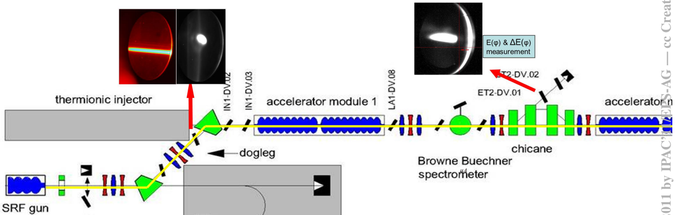
Figure 3: Layout the SRF gun and the ELBE beam line. The electron bunches extracted from the gun are guided through the achromatic dogleg and then are accelerated by the accelerator modules.
