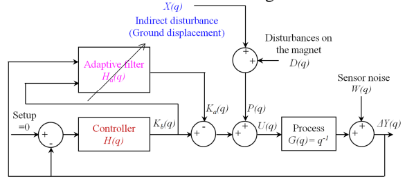
Figure 8: Adaptive feedback control scheme.
