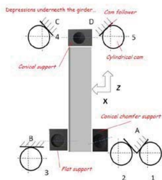
Figure 1: Configuration of cam movers.
