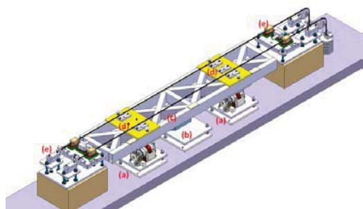
Figure 2: Description of 5 DOF setup.
