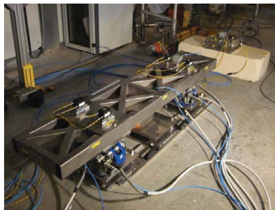
Figure 3: Blank assembly of 5 DOF setup.
