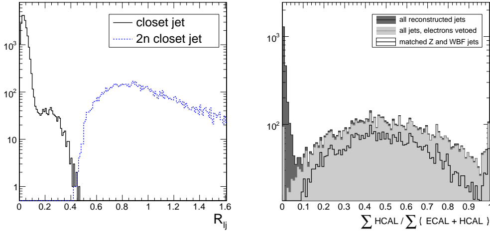
Figure 6.9. The distance R^2 = \Delta\eta^2 + \Delta\phi^2 between identified electrons and their closet jet and 2nd closet jet (left). Hadronic energy fraction of the jets reconstructed with the described iterative cone algorithm (right). The jets before (dark shaded area) and after excluding jets in a cone of size R = 0.3 around identified electrons (light shaded area) is shown together with jets matched to the generated partons (solid line). Only particles which carry at least a minimum transverse momentum of 10 GeV are considered.
