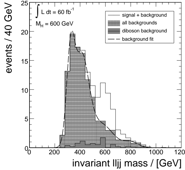
Figure 6.19. The different contributions to the background and its parameterization. Only a minor fraction of the overall background contribution (shaded histogram) arises from the WZ +jets and ZZ +jets events (dark histogram). The background is substantially dominated by Z +jets events. The shape of the background is very well described by the sum of four Gaussian distributions.
