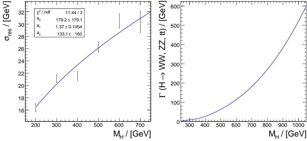
Figure 6.18. Parameterization of the Higgs boson mass resolution (left): The function \sigma(M_H)^2 = p_0 + p_1 * (M_H - p_2) is fitted to the mass resolution obtained from fast detector simulation. Calculation of the decay width as a function of the Higgs boson mass (right): Partial decay widths into weak boson and top pairs are added according to EQUATION 3.7, EQUATION 3.8 and EQUATION 3.9.
