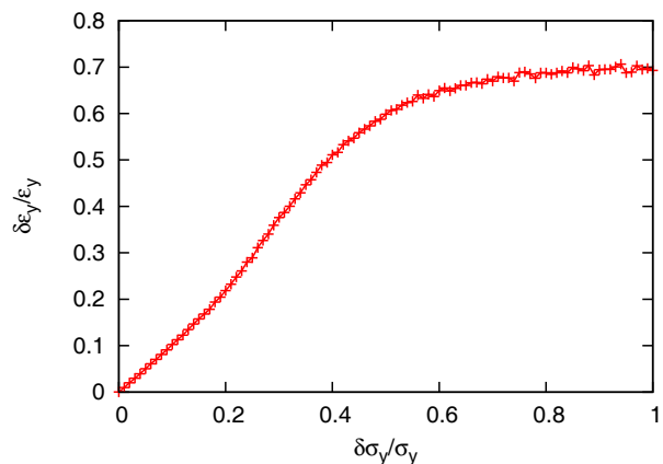
Figure 3: Relative error of the vertical emittance measurement as a function of the relative beam size measurement error.
