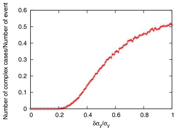
Figure 2: Fraction of simulations giving a non-physical beam matrix as a function of the beam measurement error.
