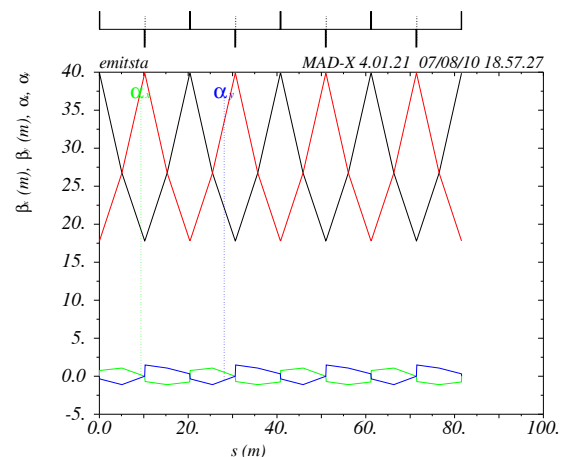
Figure 1: The optics layout of the 2D emittance measurement section.
