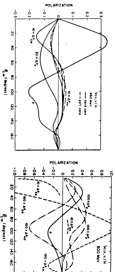
Fig. 1. Theoretical predictions for the difference in polarizations of scattered neutron and recoil proton in elastic scattering of unpolarised neutrons from unpolarised protons due to direct electromagnetic effects ( \Delta P_{EM} ), due to \rho^0 - \omega mixing ( \Delta P_{\rho\omega} ), due to the n-p mass difference effect in charged one pion exchange ( \Delta P_{\pi} ) and in \rho -exchange ( \Delta P_{\rho} ), a) by Cheung, Henley and Miller, ref. 10; b) by Gersten, ref. 11.
