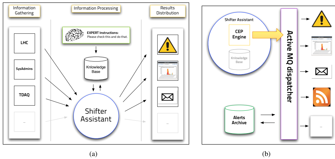
Figure 2: Shifter Assistant architecture. (a): Shifter Assistant gathers information streams from various systems and returns alerts based on patterns found in data. (b): Shifter Assistant uses ActiveMQ dispatcher system to send notifications and alerts.
