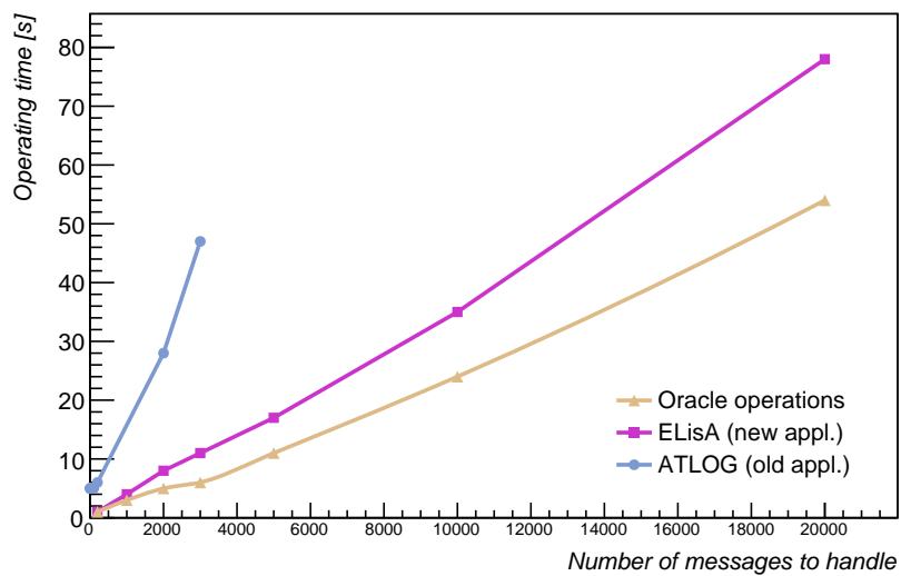
Figure 3: Speed and scalability tests of the ATLAS log message user interface
