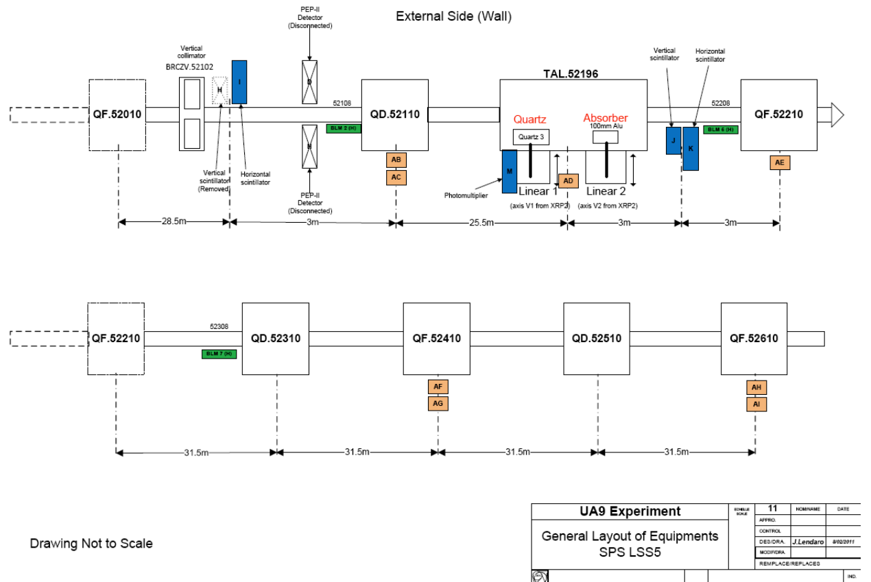
Fig 1.b) Layout of the dispersive region of UA9.
