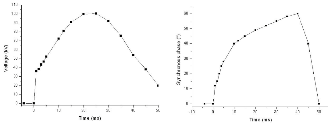
Figure 13: Synchronous phase and voltage evolution during cycle for He ions
