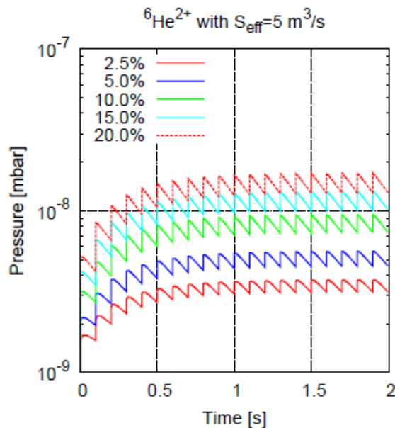
Figure 18: Pressure evolution for different losses at injection ranging from 2.5 to 20 %. The pumping speed for the calculations is S_{\text{eff}}=5 \text{ m}^3/\text{s} .
