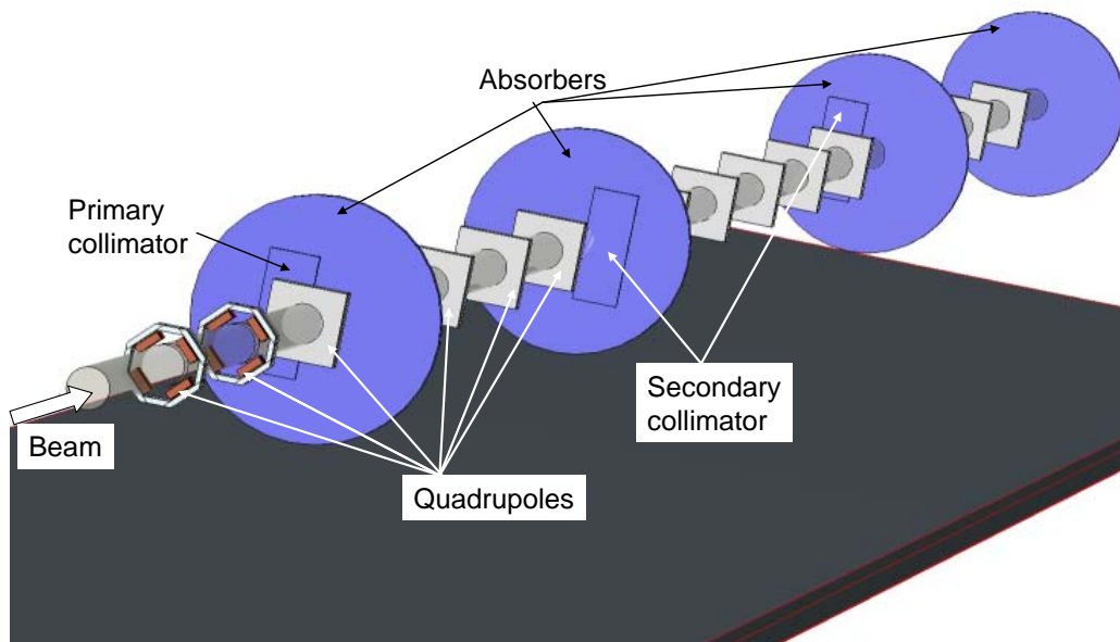
Figure 52 : Placement of graphite absorbers in the collimation section. (SimpleGeo view [38])
