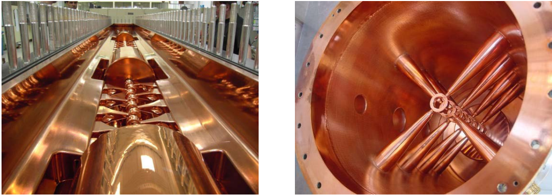
Figure 3: A 217 MHz medicine IH-DTL and the 350 MHz CH-prototype cavity for GSI.
