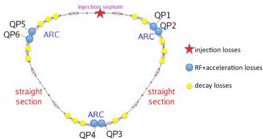
Figure 20 : Layout of the RCS. The different kinds of losses and their locations in the ring are shown.
