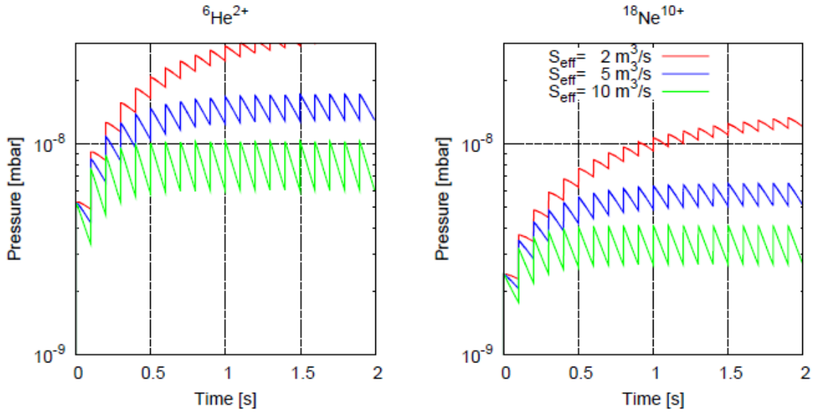
Figure 17: Pressure evolution over 20 cycles for different effective pumping speeds (2 to 10 \text{m}^3/\text{s} ) for {}^6\text{He}^{2+} (left) and {}^{18}\text{Ne}^{10+} (right).
