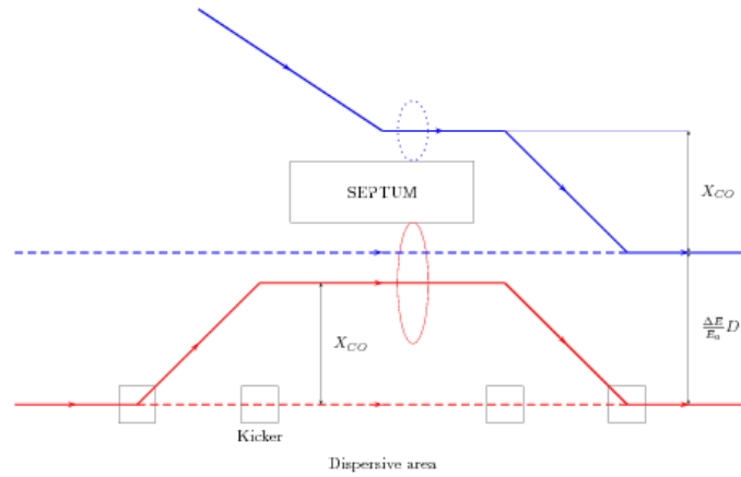
Figure 40: Injection principle. In blue, injected beam and in red, stored beam. In dashed, central axes of both beams one turn after injection (kickers off).
