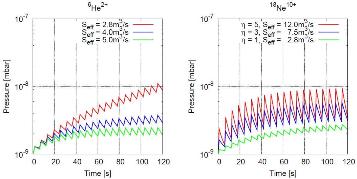
Figure 38: Pressure evolution over several cycles for {}^6\text{He}^{2+} (left) and {}^{18}\text{Ne}^{10+} (right) for different effective pumping speeds. For both projectiles the maximal available ramping rate of the SPS was assumed and for {}^{18}\text{Ne}^{10+} the cycle time was extended to 6 s. The desorption rate used for {}^6\text{He}^{2+} was \eta=10 . The rates for {}^{18}\text{Ne}^{10+} are given in the legend.
