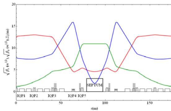
Figure 41: Optical functions in the injection section. In red/blue, horizontal/vertical betatron function and in green horizontal dispersion.
