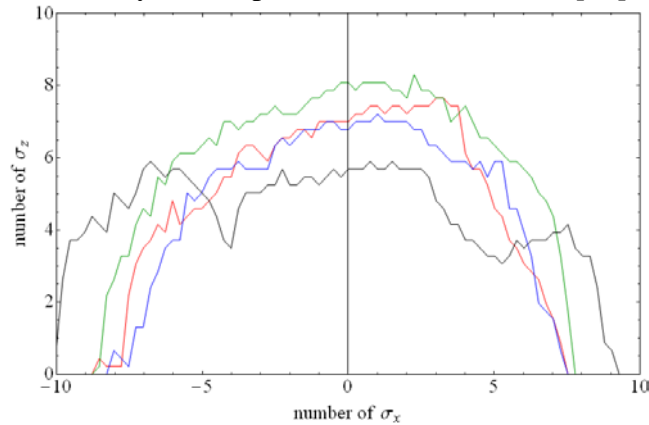
Figure 62: Dynamic aperture for 1,000 turns without optimization and after applying the fifth order (red), the seventh order (blue), the ninth order (green) or every (black) multipole component.
