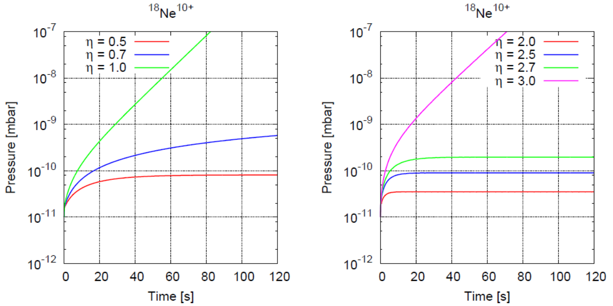
Figure 67: This figure shows the pressure evolution for ^{18}\text{Ne}^{10+} in the Decay Ring for a re-emission coefficient of 1 (left) and 0 (right). The desorption rates were varied from 0.5 to 1 and 2.0 to 3.0 respectively. All simulations were done with a starting pressure of P_0 = 10^{-11} mbar and a temperature of the cold surfaces of T = 10 K.
