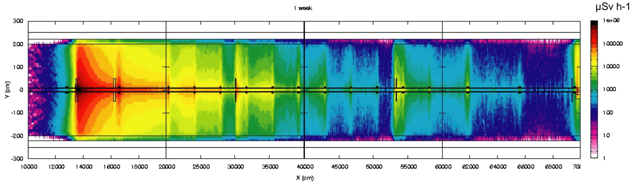
Figure 64: Residual dose rate in the straight section of the collimation section, after 1 week waiting time and 3-month ^{18}\text{Ne} irradiation.
