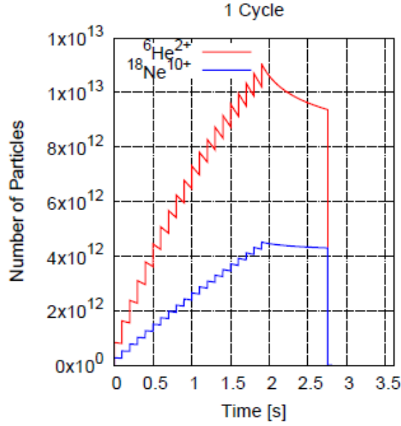
Figure 26: Number of particles over one cycle for {}^6\text{He}^{2+} and {}^{18}\text{Ne}^{10+} .
