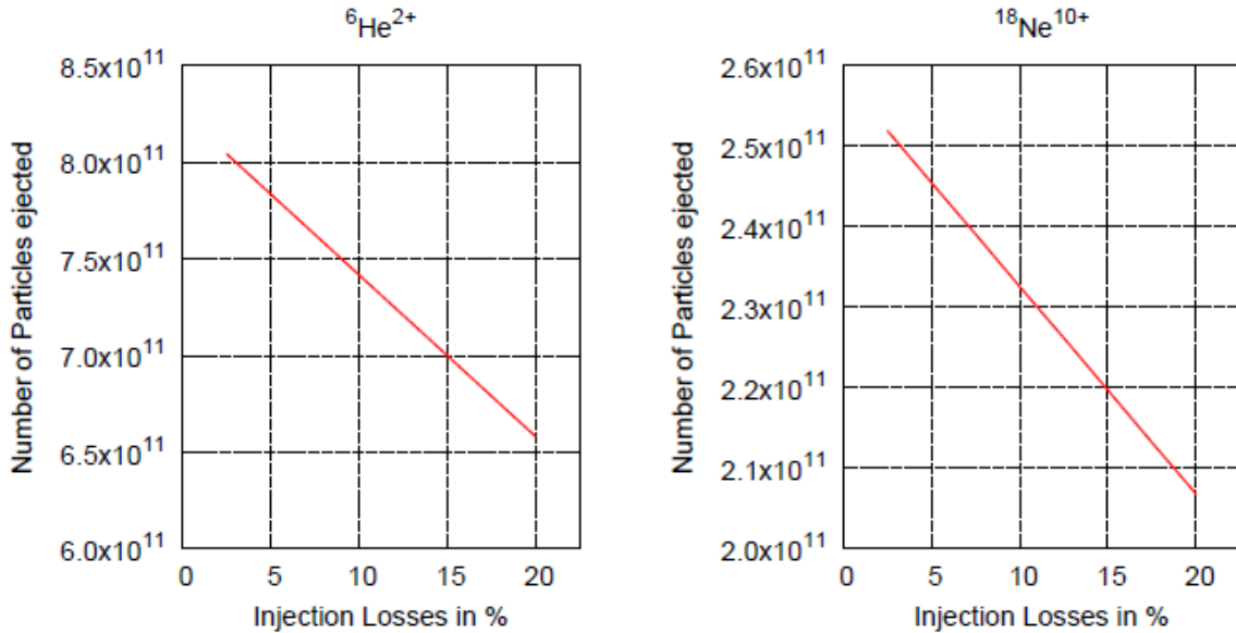
Figure 16: Number of ejected particles against beam losses at injection for an effective pumping speed of S_{\text{eff}}=5 \text{ m}^3/\text{s} for {}^6\text{He}^{2+} (left) and {}^{18}\text{Ne}^{10+} (right).
