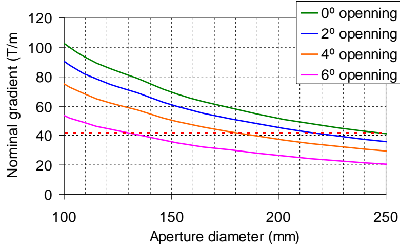
Figure 59 : Parametric dependence of quadrupole gradient on aperture for different midplane opening angles.
