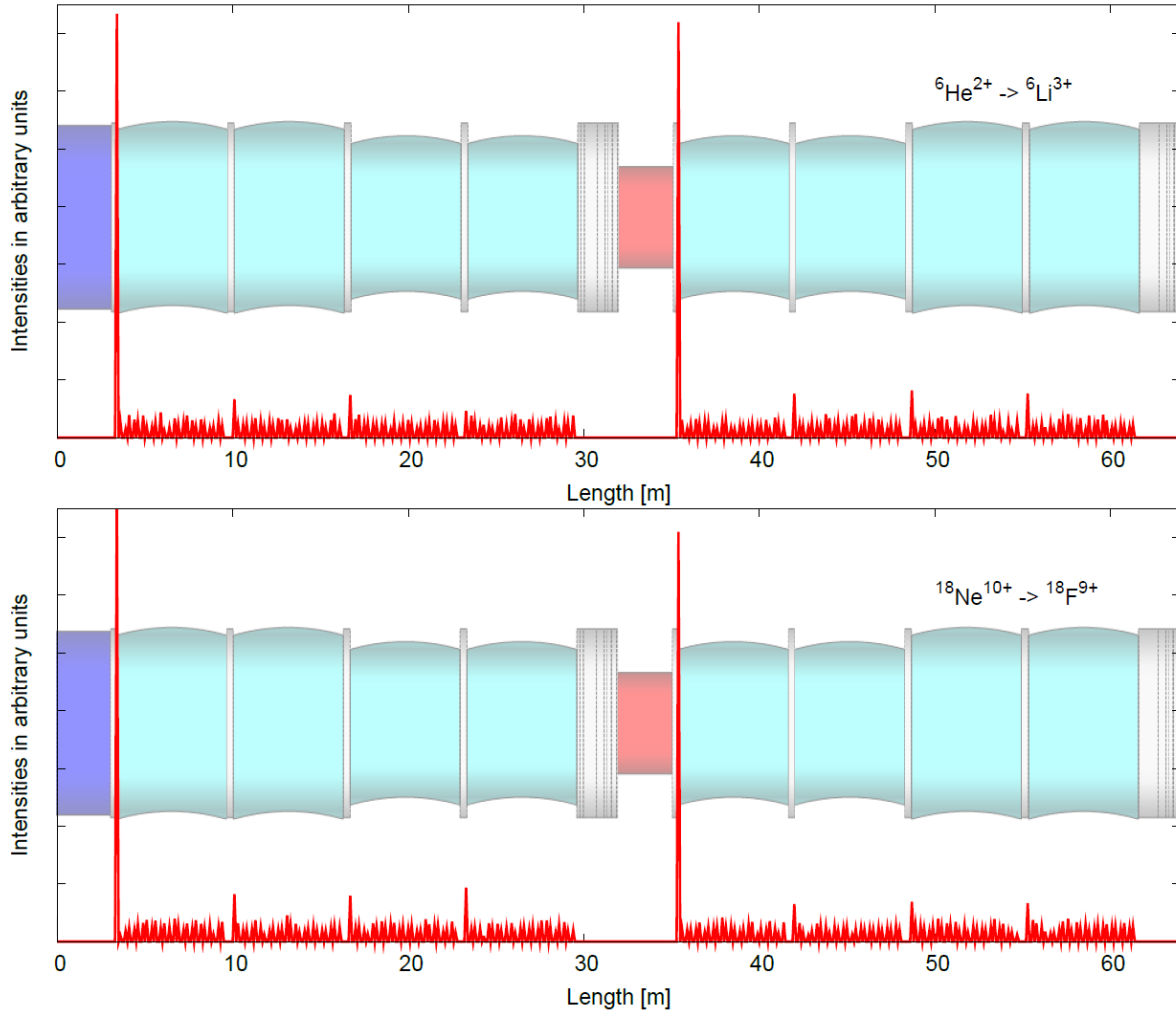
Figure 35: Loss distribution {}^6\text{He}^{2+} \rightarrow {}^6\text{Li}^{3+} (top) and {}^{18}\text{Ne}^{10+} \rightarrow {}^{18}\text{F}^{9+} (bottom) at injection energy. Dipole magnets are shown in light blue, quadrupole magnets in red and blue.
