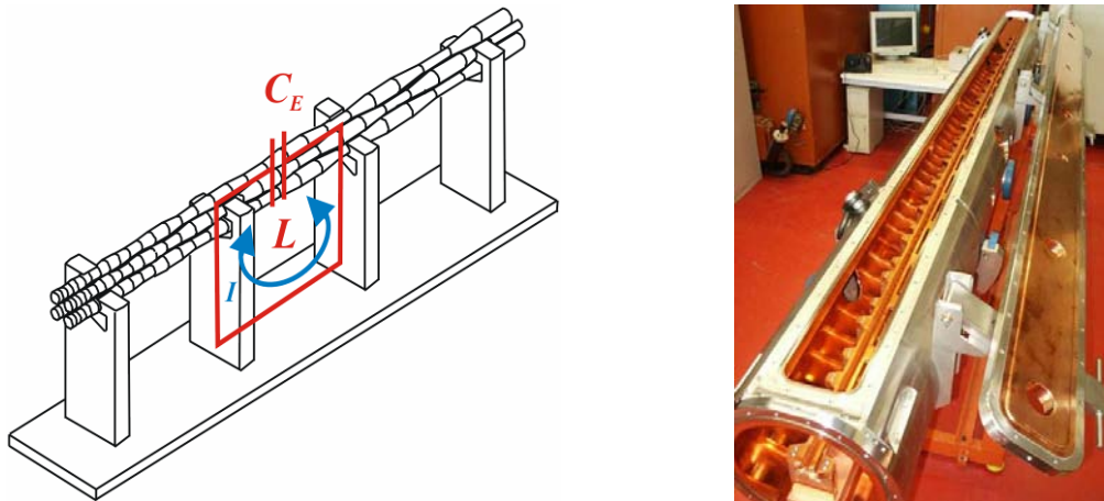
Figure 2: Scheme of the 4-rod-RFQ on the left and - as an example - the SARAF 176 MHz 4-rod RFQ built by NTG Company on the right
