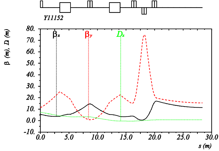
Figure 6 : Lattice functions for a quarter of the cooler ring. The electron cooler would be in the right part of the diagram.
