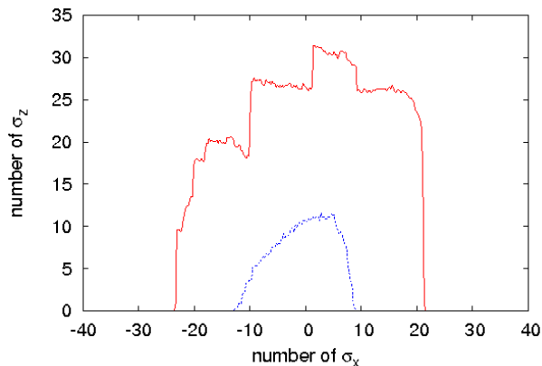
Figure 60: Dynamic aperture for 10,000 turns at the middle of the injection insertion. In red, with 6 sextupole families and in blue with 2 sextupole families.
