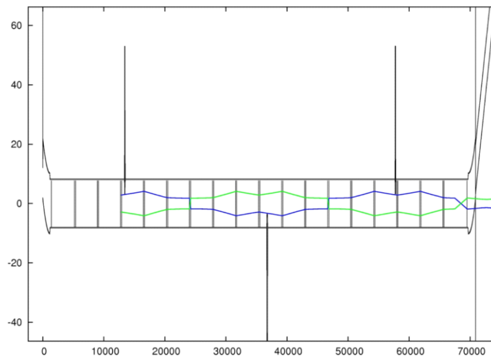
Figure 50 : Placement of the primary and secondary collimators along the collimation section. The x and z axis are in meters, and the blue and green lines are the limits of the beam envelope for a beam emittance of 2.6\pi\text{mm.mrad} and maximum \delta=2.5\text{‰} .
