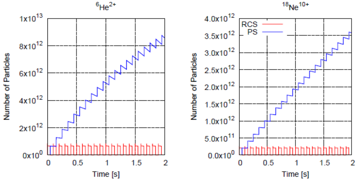
Figure 15: Number of particles over twenty cycles for {}^6\text{He}^{2+} (left) and {}^{18}\text{Ne}^{10+} (right). The blue line shows the accumulation of the particles within the PS.
