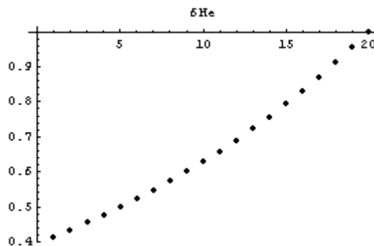
Figure 24: Relative helium intensity along the bunch train in the PS.
