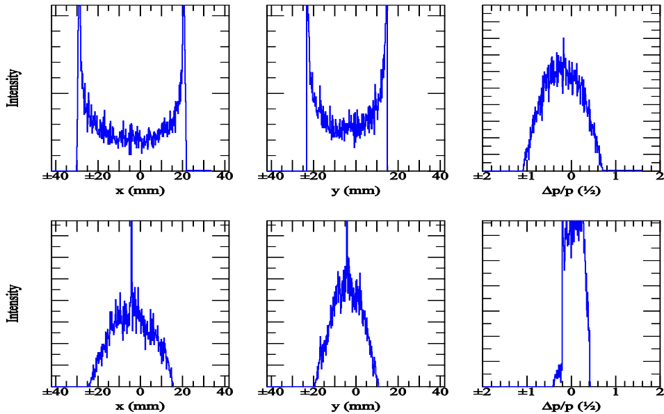
Figure 7 : Simulation of horizontal, vertical, and longitudinal profiles of an ^{18}\text{Ne}^{10+} beam before (above) and after (below) 0.1 s cooling. Initially all ions have the same emittances, \epsilon_x=65 \pi mm mrad and \epsilon_y=30 \pi mm mrad. Intrabeam scattering is not included so after cooling the central peak becomes unrealistically high.
