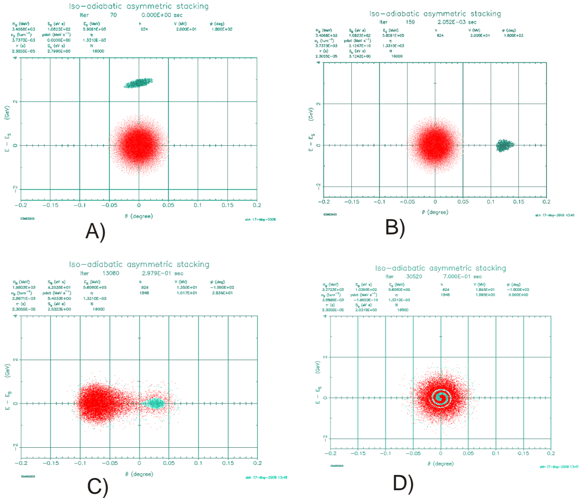
Figure 43 : The four phases of the bunch merging for {}^6\text{He} as simulated by ESME. A) off-momentum injection. B) rotation in the longitudinal phase space (synchrotron motion). C) asymmetric bunch merging. D) symmetric merging leading to the insertion of the fresh bunch into the center of the stored one.
