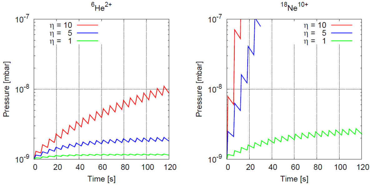
Figure 37 shows that this measurement would slow down the pressure rise for {}^6\text{He}^{2+} operation with \eta=10 and stabilize the {}^{18}\text{Ne}^{10+} operation with \eta=1 . In this scenario accelerating {}^{18}\text{Ne}^{10+} ions with \eta>1 is still not feasible. In the following paragraph the effect of an increased effective pumping speed will be discussed.
