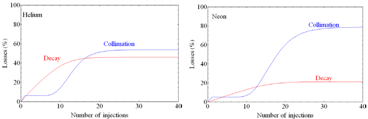
Figure 48: Loss amount as a function of time for Helium (left) and Neon (right).
