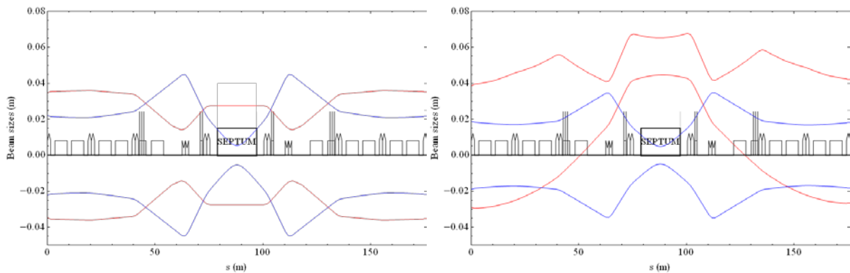
Figure 42: On left, sizes of the stored beam at 6 sigma in the injection insertion. On right, sizes of the injected beam at 5 sigma in the injection insertion. In red, beam sizes in the horizontal plan and
