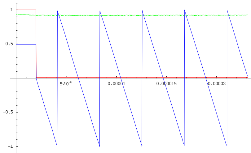
Figure 47: Mathematica simulation of one revolution period with heavy transient beam loading, assuming a period of 23 \mu\text{s} and a beam current of 100 A over 2 \mu\text{s} . Total current (beam + generator) in units of 100 A (red); phase of this current in units of \pi (blue); the resulting gap voltage in units of 300 kV (green).
