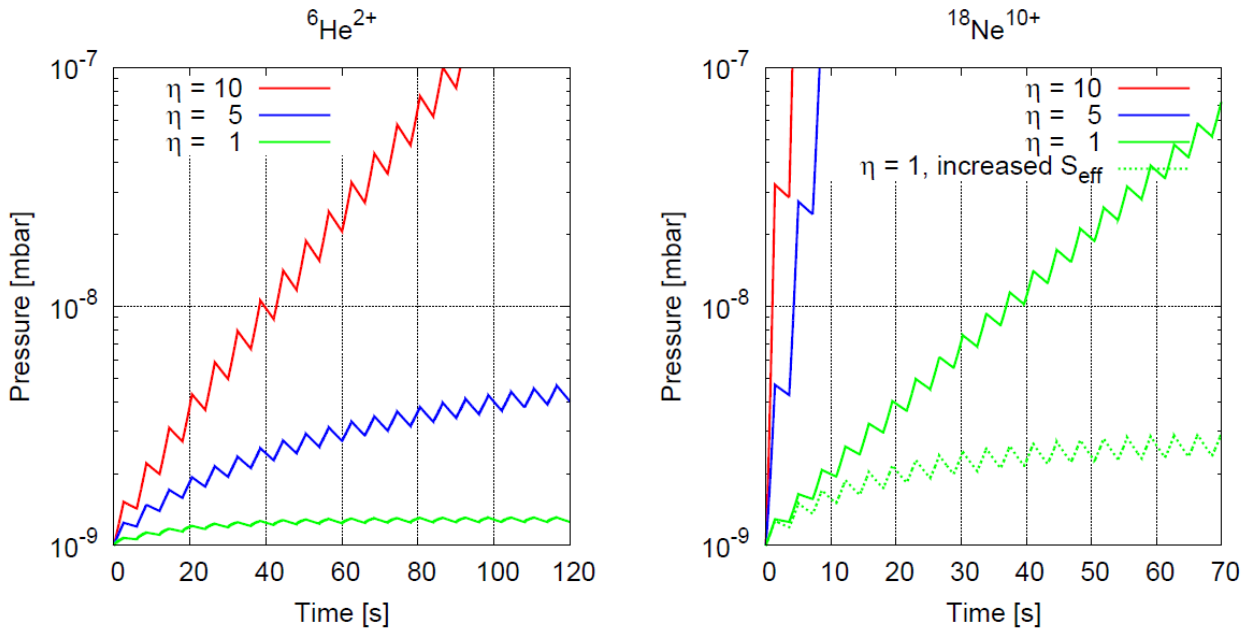
Figure 36: Pressure evolution over several cycles for {}^6\text{He}^{2+} (left) and {}^{18}\text{Ne}^{10+} (right) for different desorption rates using the proposed cycle. For {}^{18}\text{Ne}^{10+} there is one simulation with an increased effective pumping speed of 7.5 \text{ m}^3/\text{s} .
