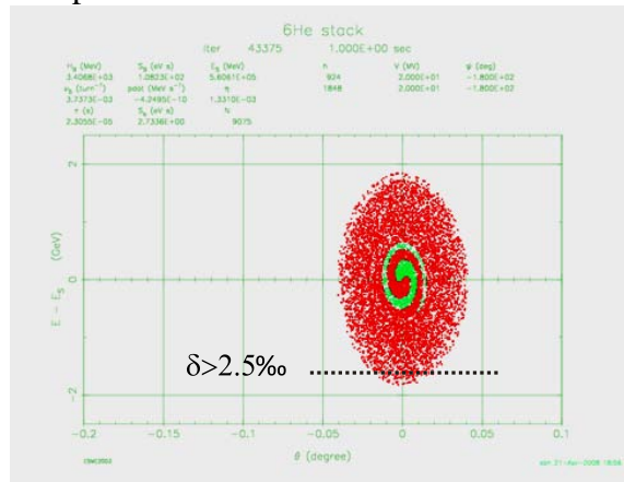
Figure 49: {}^6\text{He} bunch phase space stretching after the ramping up of the second harmonic, as calculated by ESME.
