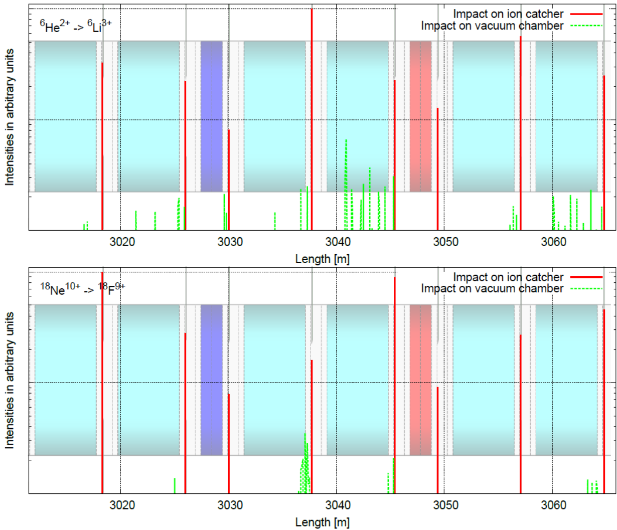
Figure 65: Loss distribution for {}^6\text{He}^{2+} \rightarrow {}^6\text{Li}^{3+} (top) and {}^{18}\text{Ne}^{10+} \rightarrow {}^{18}\text{F}^{9+} (bottom) at injection energy. Dipole magnets are shown in light blue, quadrupole magnets in red and blue and ion catchers as gray lines. The peaked distribution of ions hitting the vacuum chamber is due to the low number of tracked particles (see text). Note that the intensities are scaled logarithmically.
