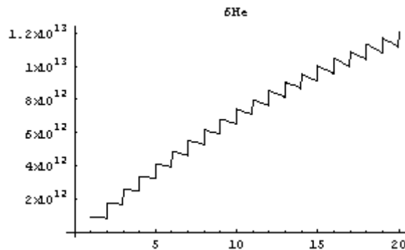
Figure 23: Number of helium ions accumulated in the PS versus RCS batches.
