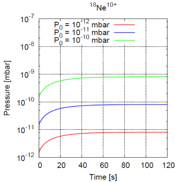
Figure 68: The figure shows the pressure evolution for ^{18}\text{Ne}^{10+} assuming a desorption rate of \eta = 2.7 and a re-emission coefficient of 0. The temperature was set to T = 10 K.
