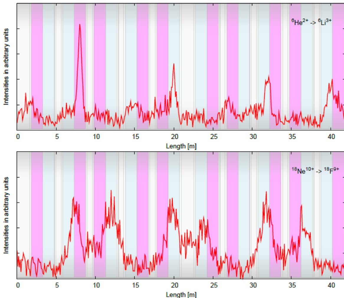
Figure 25: Loss distribution for {}^6\text{He}^{2+} \rightarrow {}^6\text{Li}^{3+} (top) and {}^{18}\text{Ne}^{10+} \rightarrow {}^{18}\text{F}^{9+} (bottom) at injection energy. The combined function magnets are shown in light blue/magenta.
