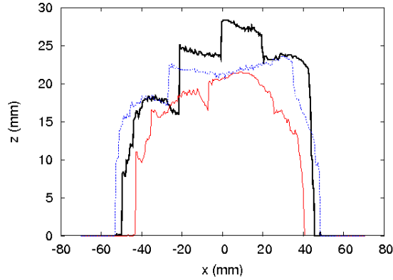
Figure 61: Dynamic aperture around the chromatic orbit for 10,000 turns at the middle of the injection insertion. In black, at \delta=0 , in red at \delta=2.5\% and in blue at \delta=-2.5\% .
