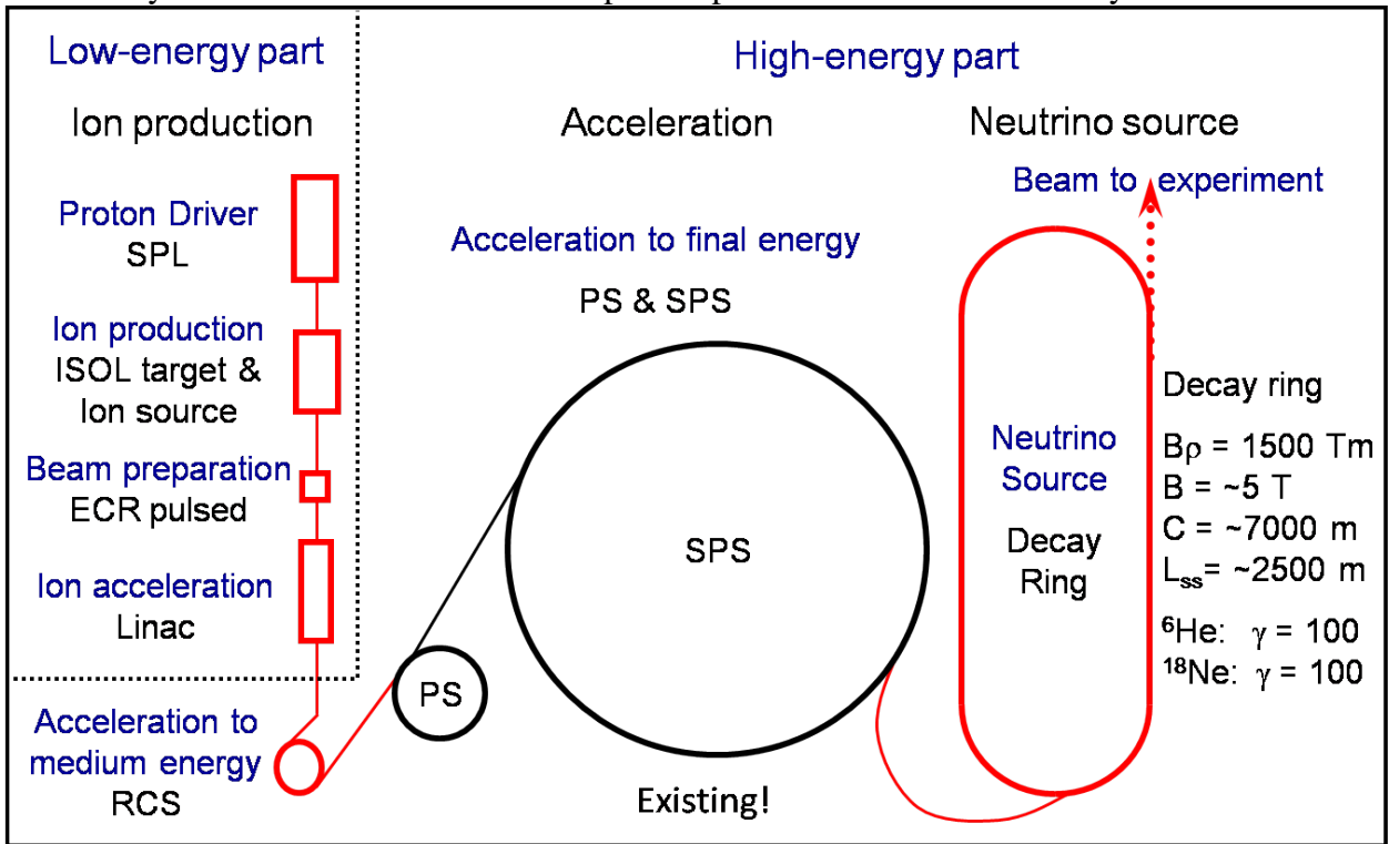
Figure 1: Overview of the CERN-baseline Beta-Beam.
