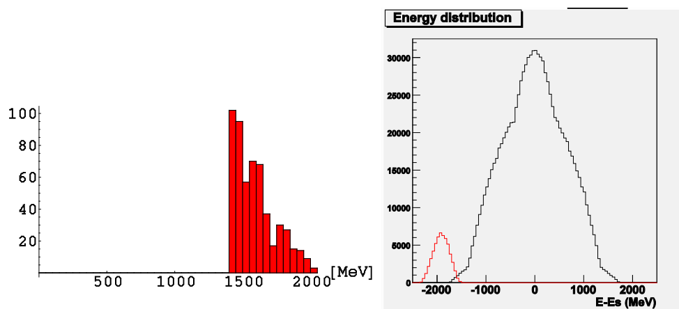
Figure 51 : Left: energy spread of the collimated {}^6\text{He} halo as estimated by ESME. Right: energy spread of the merged bunch before the ramping up (in black) energy spread of the collimated {}^6\text{He} halo as after the ramping up (in red), as calculated by ACCSIM.
