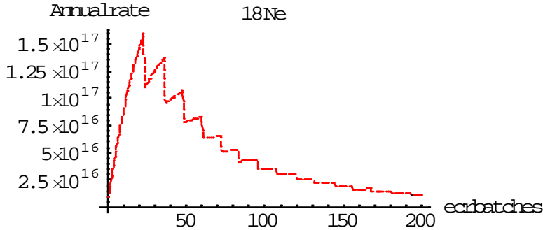
Figure 9 : The annual rate of neutrinos along one straight section of the decay ring as a function of the number of pulses from the linac that are accumulated in the accumulator ring. A total of 10 bunches from the accumulator ring is stored in the SPS before further acceleration and injection into the decay ring. The discontinuities in the curve are due to a requirement that the PS and SPS cycle time must be a multiple of 1.2 seconds.
