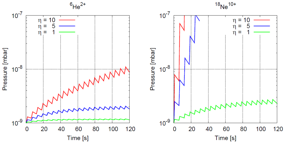
Figure 37: Pressure evolution over several cycles for {}^6\text{He}^{2+} (left) and {}^{18}\text{Ne}^{10+} (right) for different desorption rates using the maximal available ramping rate and extending the {}^{18}\text{Ne}^{10+} cycle to 6 s.
