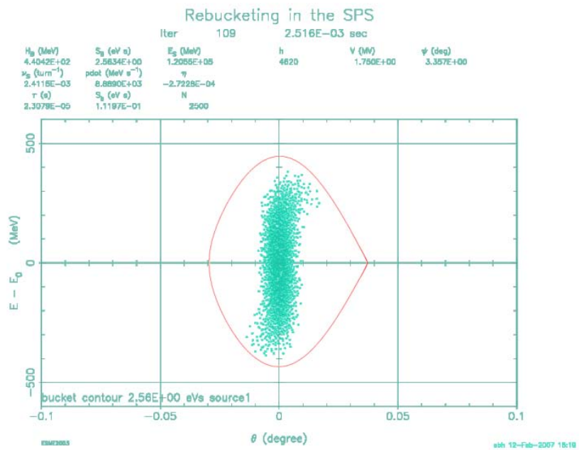
Figure 31: The bunch of Fig. 9 after the 40 MHz bucket is superseded by a 1.75 MV, 200 MHz one.
