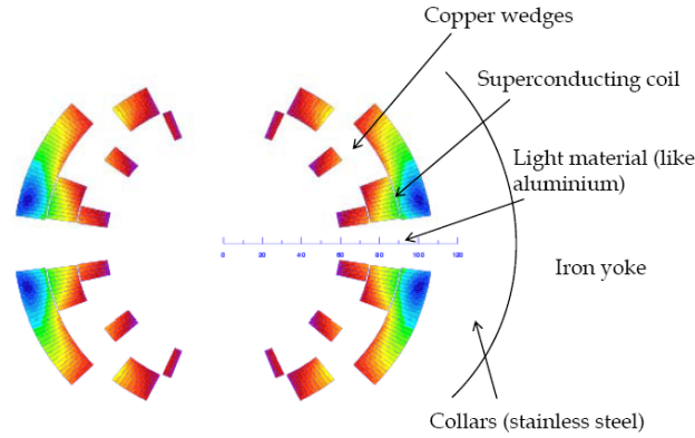
Figure 57 : Transverse cross-section of the coil of an open mid-plane dipole magnets for the beta-beam decay ring.
