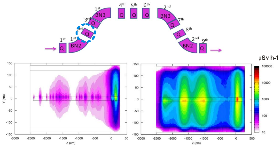
Figure 63: Residual dose in the 2^{\text{nd}} quadrupole of the first bump of the collimation section after 3 month of irradiation and 1 week waiting time. The upper picture represents the magnets arrangement within the first bump. Left bottom: residual dose map for {}^6\text{He} , right bottom: residual dose map for {}^{18}\text{Ne} .
