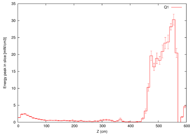
Figure 54 : Peak energy deposition in each longitudinal bin along the superconducting cable on the dipole D2 in the lattice cell. Recommended limit value for quenching is 4.3 \text{ mW/cm}^3 . The bars represent statistical errors.
