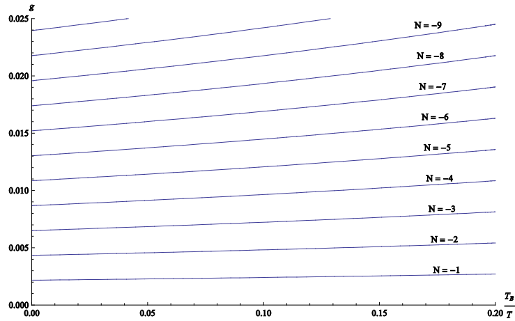
Figure 46: Discrete values of g as function of T_B/T for harmonic 924.
