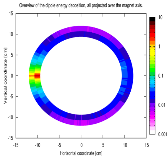
Figure 55 : Overview of the energy distribution in the superconducting cable on the dipole 3 in the lattice cell. The superconducting cable is modeled, for simplicity, as a cylinder. Transverse projection, averaged over the length of the magnet.
