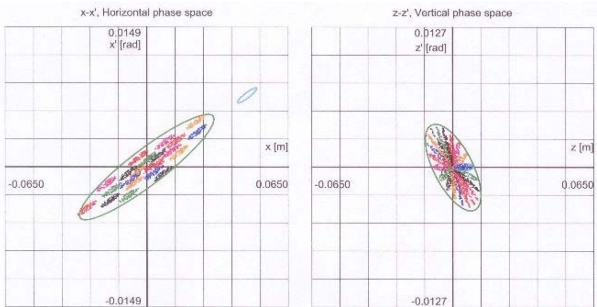
Figure 12: Phase space distributions of the multi-turn injected beam (left : horizontal plane, right : vertical plane)
