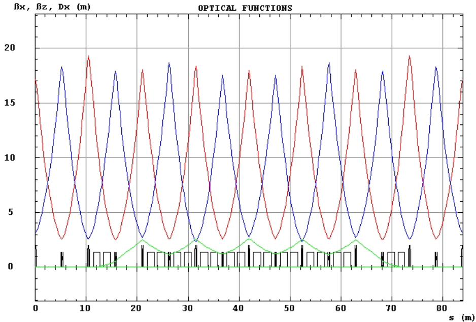
Figure 11: Optical functions for one superperiod
