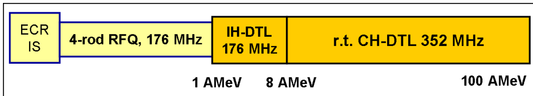
Figure 4: Schematic layout of an IH/CH-DTL for the production of \beta -beams.
