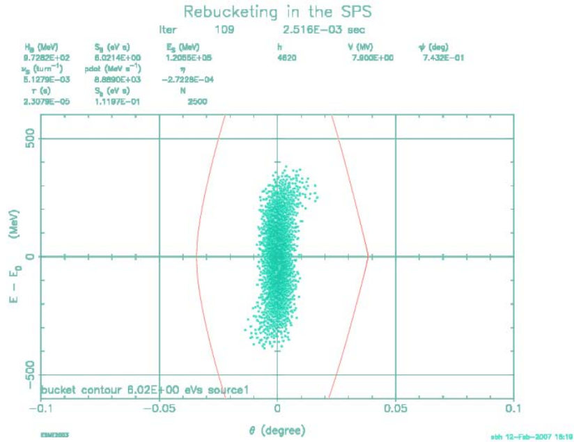
Figure 33: The bunch of Fig. 11 after a step in 200 MHz voltage to 7.9 MV. A small fraction of the bunch population remains at large amplitude.
