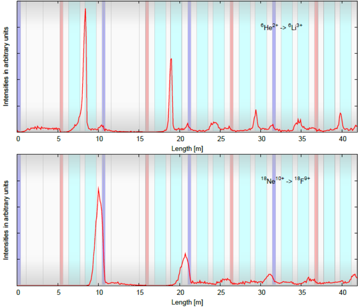
Figure 14: Loss distribution for {}^6\text{He}^{2+} \rightarrow {}^6\text{Li}^{3+} (top) and {}^{18}\text{Ne}^{10+} \rightarrow {}^{18}\text{F}^{9+} (bottom) at injection energy. Dipole magnets are shown in light blue, quadrupole magnets in red and blue.
