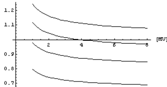
Figure 29: Ratio of 40 MHz bunch length to 200 MHz bucket length versus 200 MHz voltage for helium ions at \gamma=19, 20, 21, 22 (from top to bottom) and a ramp rate of 0.02 T/s in the SPS.
