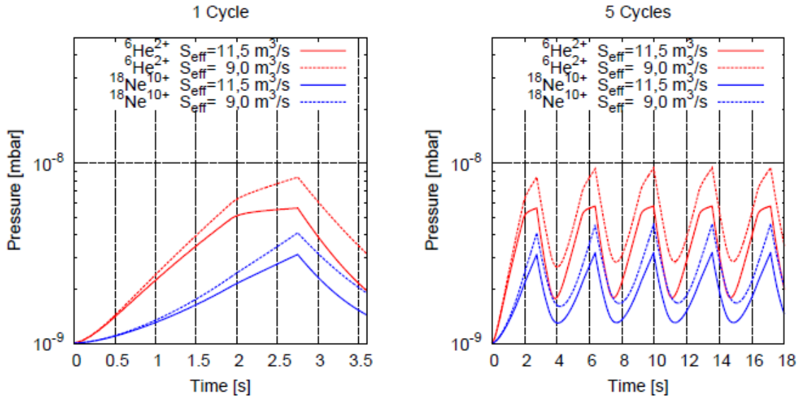
Figure 27: Pressure over one and five cycles for different effective pumping speeds (11.5 and 9.0\text{m}^3/\text{s} ) for {}^6\text{He}^{2+} and {}^{18}\text{Ne}^{10+} .
