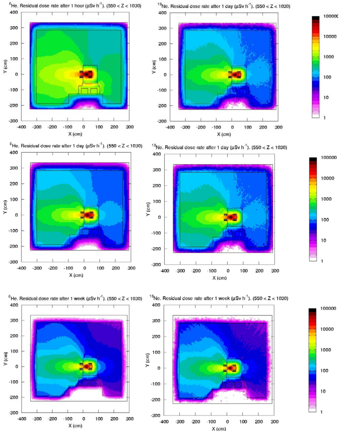
Figure 28 :From top to bottom: ambient dose equivalent rate after 3 month irradiation followed by
