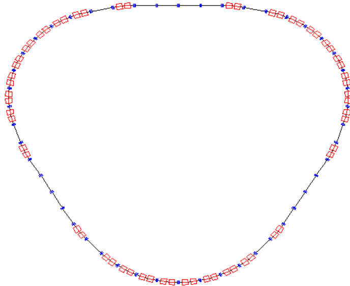
Figure 10: Schematic layout of the RCS
