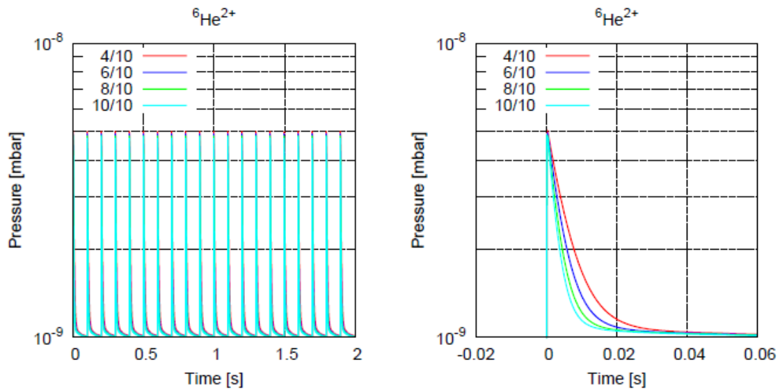
Figure 19: Pressure evolution with NEG-coated dipole chambers. The projectile ion is {}^6\text{He}^{2+} and the pumping speed is S_{\text{eff}}=5 \text{ m}^3/\text{s} . The number of NEG-coated dipole doublets per arc was altered in the range from 4 to 10 for the different lines.
