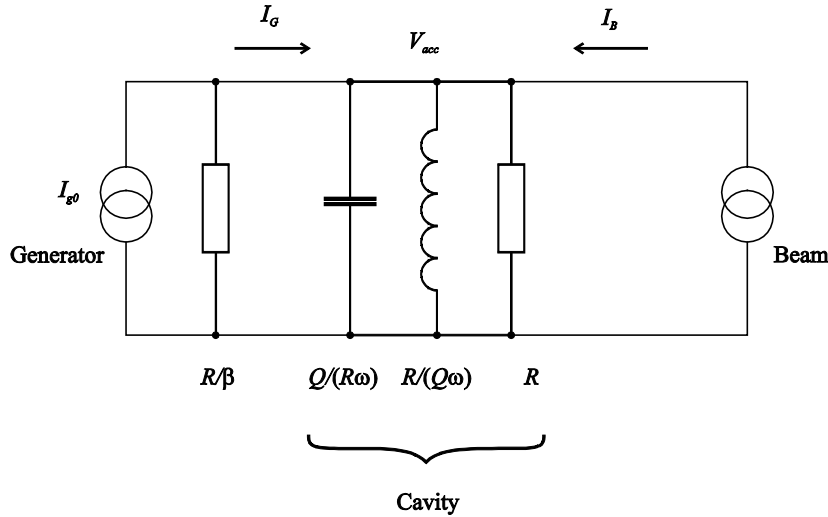
Figure 44: Equivalent circuit of a cavity including beam loading.
