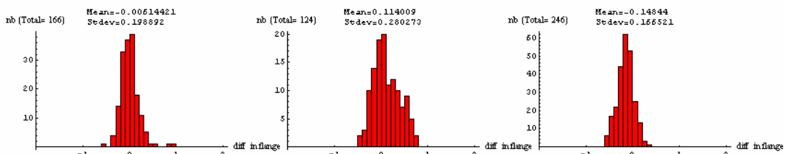
Figure 9: Situation of the horizontal position of the flange at CERN, top firm 1, middle firm 2 and bottom firm 3 (all magnets cold tested and with central support blocked).
