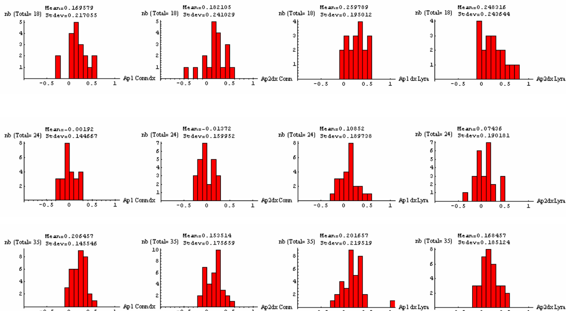
Figure 9: Situation of the horizontal position of the flange at CERN, top firm 1, middle firm 2 and bottom firm 3 (all magnets cold tested and with central support blocked).
