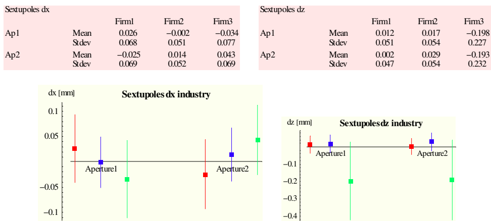
Figure 12: Sextupole positions in industry. The vertical bars correspond to \pm 1 standard deviation. Red, blue and green represent firm 1, 2 and 3 respectively.
