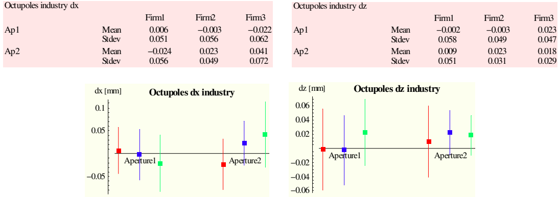
Figure 14: Octupole positions in industry. The vertical bars correspond to \pm 1 standard deviation. Red, blue and green represent firm 1, 2 and 3 respectively.
