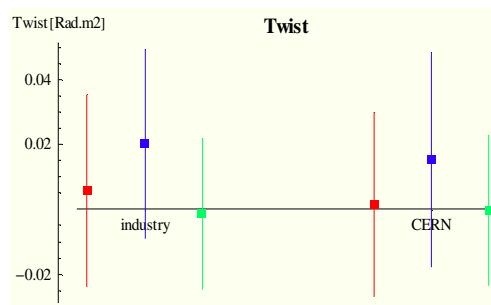
Figure 17: The twist of the magnet at industry and at CERN. Red, blue and green represent firm 1, 2 and 3 respectively.
