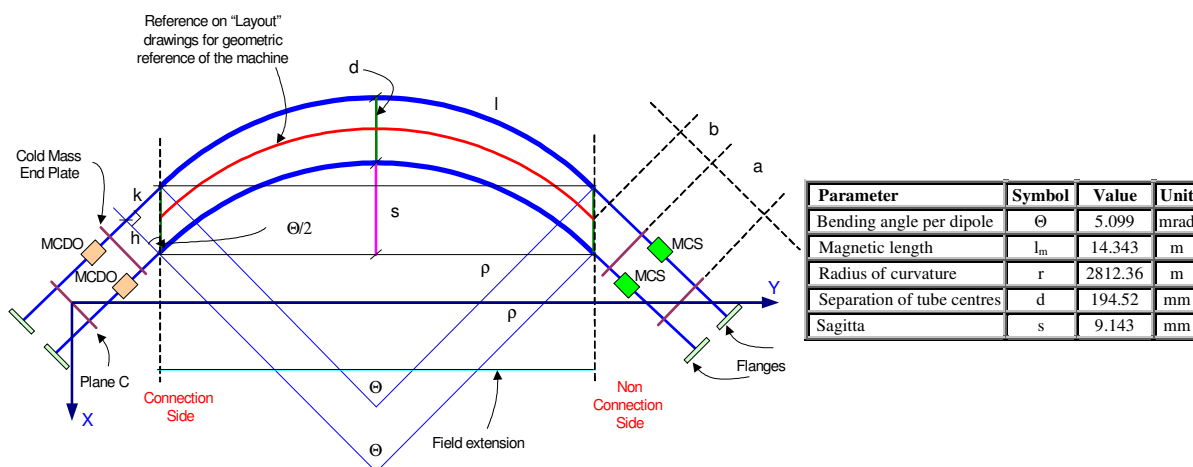
Figure 2: The theoretical geometry of the dipole and some important geometry values (warm conditions). The measurements extend roughly from “Plane C” (C stands for connection) to the corresponding plane at the Non Connection side. The coordinate system is right handed and the vertical direction, z, ideally points opposite gravity.
