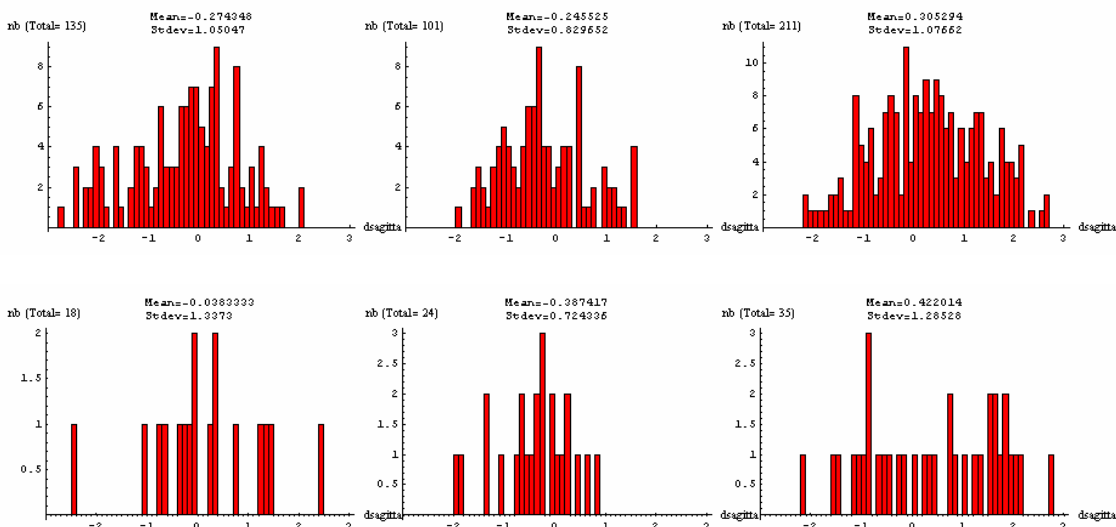
Figure 4: The sagitta with respect to the nominal sagitta in industry from left to right for firm 1, 2 and 3 (top graphs) and at CERN, measured after cold test with central support adjusted like in industry, from left to right for firm 1, 2 and 3 (bottom graphs).
