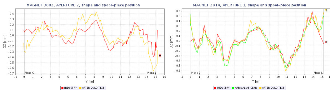
Figure 7: Examples of measurements in the vertical plane: to the left a magnet not perfectly aligned, to the right a magnet well aligned but showing anomalies at the ends. The effect is present also at arrival at CERN.
