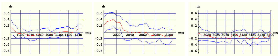
Figure 11: The difference in the vertical flange position between industry and the first measurement after cold test: for each 5 th magnet the moving average of 15 preceding magnets is plotted. In red, the mean, in blue, the standard deviation. From left to right firm 1, 2 and 3.
