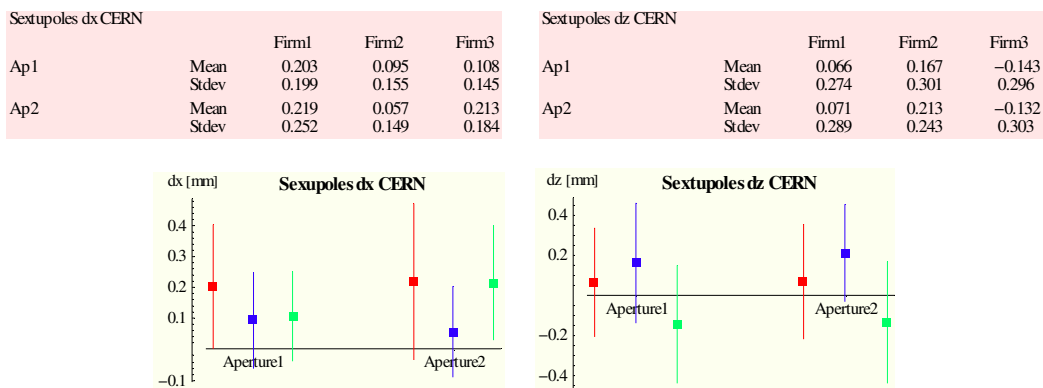
Figure 13: Sextupole positions (estimated) at CERN after cold test and with central support blocked. The vertical bars correspond to \pm 1 standard deviation. Red, blue and green represent firm 1, 2 and 3 respectively.
