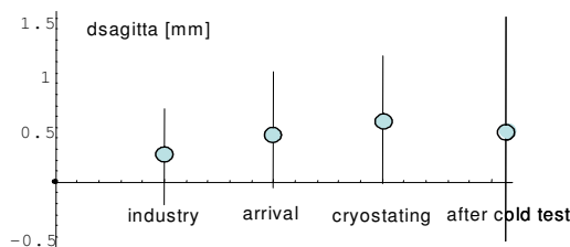
Figure 3: The evolution of the dsagitta for magnets without blocking of the central support. The measurements are from industry from arrival at CERN from after cryostating and finally from after cold testing. The vertical bars correspond to \pm 1 standard deviation.
