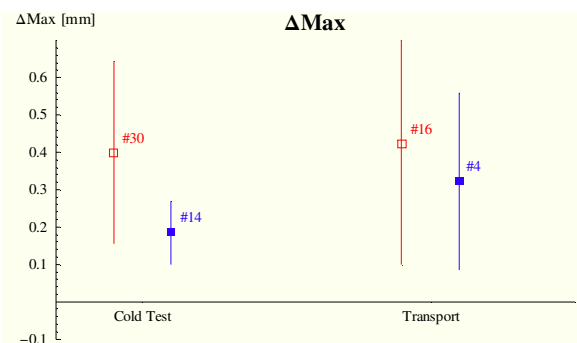
Figure 6: The maximum change in the shape before and after cold test (left) and during transport on the CERN site (right). Red: not blocked magnets, blue blocked magnets. The vertical bars correspond to \pm 1 standard deviation.
