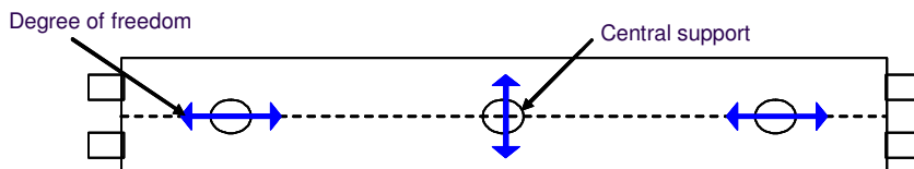
Figure 1: The supporting of the cold mass of the LHC main dipole. The two external supports allow movements in the longitudinal direction. The central support was originally designed to allow lateral movements as shown in the figure, but is now blocked laterally.
