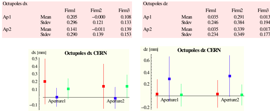
Figure 15: Octupole positions at CERN (estimated). The vertical bars correspond to \pm 1 standard deviation. Red, blue and green represent firm 1, 2 and 3 respectively.
