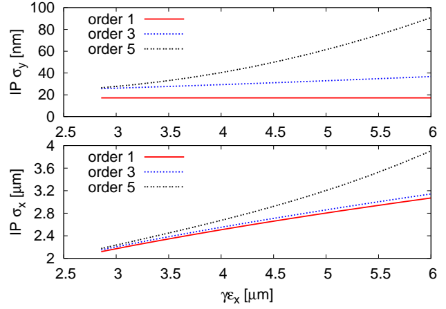
Figure 3: (top): Vertical beam size \sigma_y at the IP versus horizontal emittance for three different orders: first, third and fifth. Clearly the fifth order amplify dramatically the beam size. (bottom): Horizontal beam size \sigma_x at the IP versus horizontal emittance
