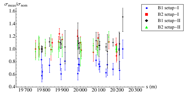
Figure 2: Ratio between nominal beam sizes and beam sizes found during the collimation setups at collimators in IR7.
