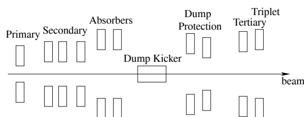
Figure 1: Simplified sketch of the gap opening arrangement of collimator classes normalized by beam size.
