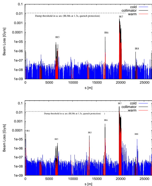
Figure 3: Horizontal betatron losses in B1 generated by crossing a 1/3 integer tune resonance. Blue/red/black bars indicate losses in the cold aperture/ warm aperture / collimators. Top: setup-I; Bottom: setup-II.
