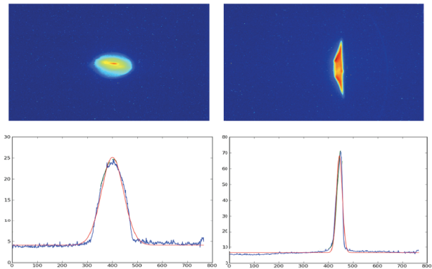
Figure 6: Examples of YAG images of the beam with corresponding intensity profiles and Gaussian fits. The left shows the upstream YAG image, the right the downstream YAG after the vertical slit has been inserted in place of the upstream screen.
