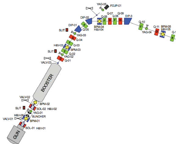
Figure 1: Layout of the ALICE injector. A 350 kV DC GaAs photocathode is followed by a 2-solenoid emittance matching section, buncher, and 2-cavity TESLA-type accelerating module [8].
