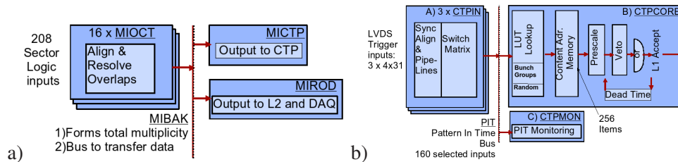
Figure 1. Outline of the a) MUCTPI and b) CTP boards.
