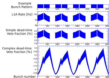
Figure 4. Example of a close to nominal LHC bunch pattern, LIA rate and dead-time (both simple and complex) veto, as measured by the CTP counters.
