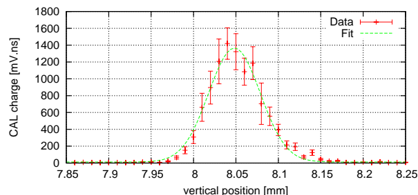
Figure 6: Vertical scan ( \sigma_y = 30.38 \pm 1.43\mu\text{m} ).
