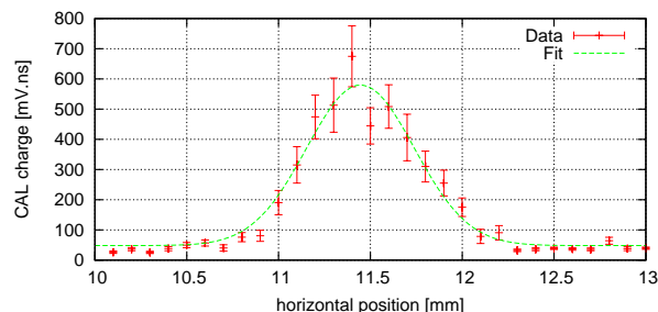
Figure 7: Horizontal scan ( \sigma_x = 293.6 \pm 18.1\mu\text{m} ).
