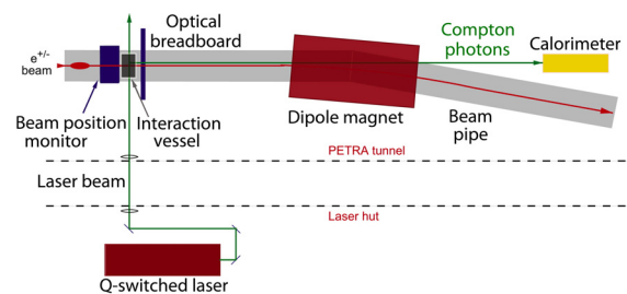
Figure 2: Overview of the LW setup [1].
