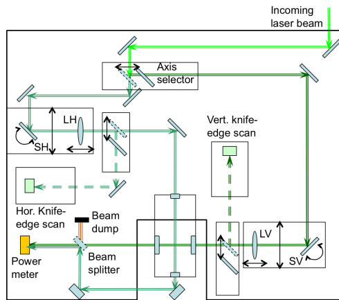
Figure 3: Schematic layout of the vertical breadboard.
