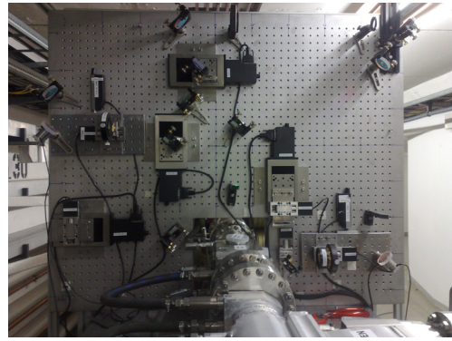
Figure 4: Photo of the LW optical breadboard.
