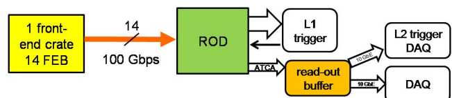
Figure 7: Possible back-end architecture of the upgraded LAr read-out.
