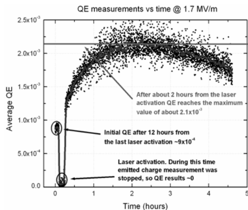
Figure 3: QE of Mg thick sample vs. time after the laser cleaning.
