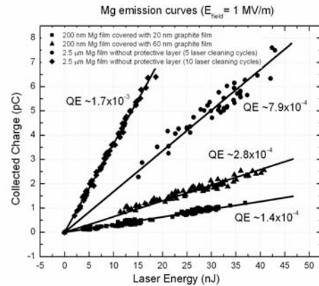
Figure 1: Highest achieved QE values for various PLD Mg grown samples.
