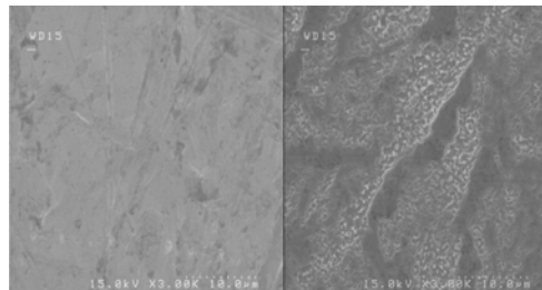
Figure 5: Left picture: as deposited Pb sample; Right: after laser cleaning
