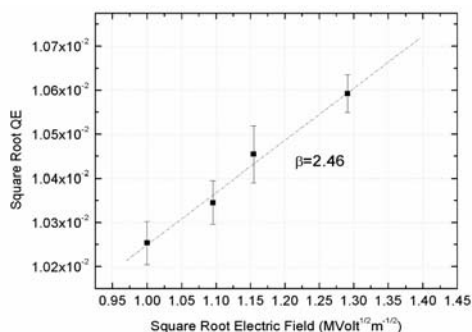
Figure 4: Pb sample QE vs. extraction field and \beta evaluation.
