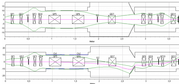
Figure 3 : Vertical envelopes in the chopper-line
