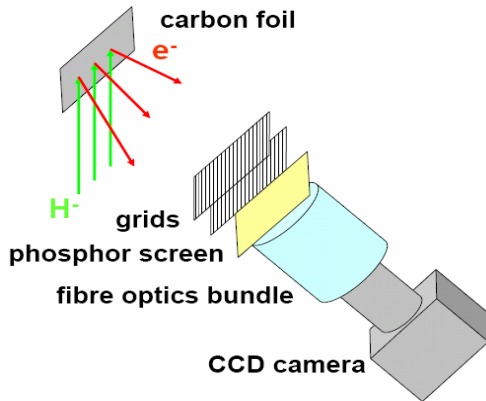
Figure 5 : BSHM hardware
