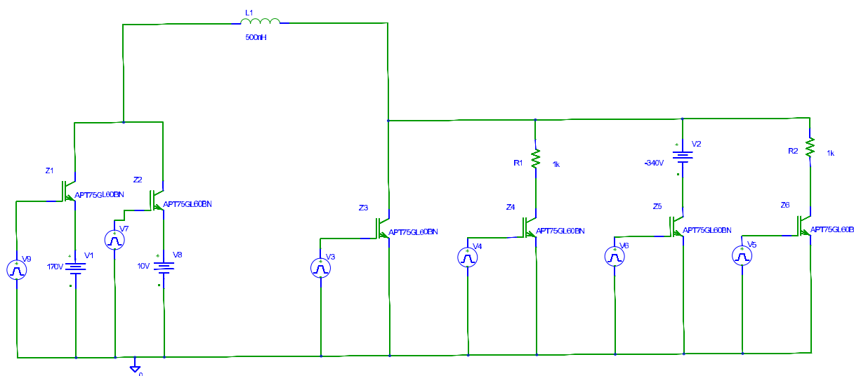
Figure 6: Circuit diagram in SPICE [7].
