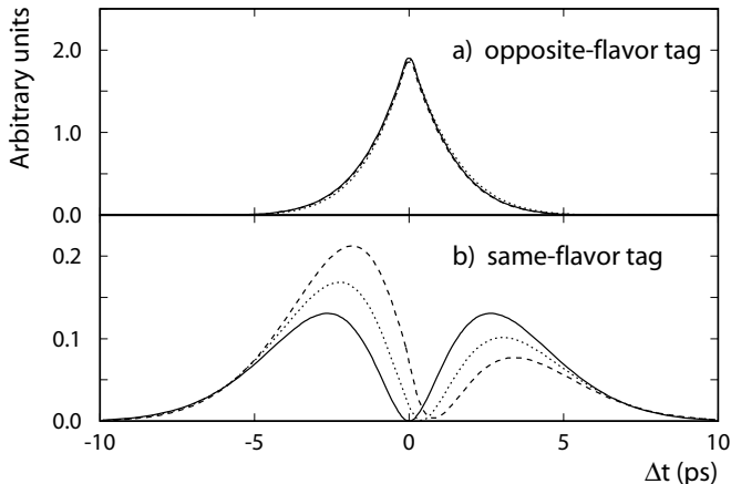
Figure 5.1: Time-dependent decay distributions for the final state D^{*-}\pi^+ , for a) a \bar{B}^0 tag, and b) a B^0 tag. The angle (2\beta + \gamma) is set to the value 1.86. The situation with no doubly-CKM-suppressed contribution on both the tag-side and reconstruction-side is indicated with the solid curve. The dotted curve has r = 0.1 and \delta = 0 , but no tag-side interference. The dashed curve represents the example with r = r' = 0.1 , \delta = 0 , and \delta' = \pi . In these examples, the r and r' values are \times 5 the expected values in order to clearly illustrate the differences with respect to the case with r = r' = 0 .
