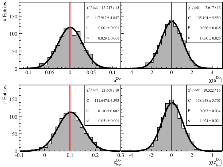
Figure 7.14: Fitted a and c_{lep} parameters of B \rightarrow D \rho sample. The generated CP asymmetry: a = 0 , and c_{lep} = 0.10 .
