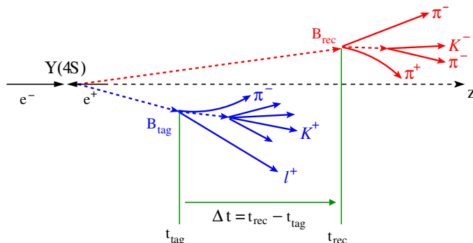
Figure 2.12: The decay Y(4S) \rightarrow B^0 \bar{B}^0 , where one B decays to the final state D^{*-} \pi^+ , B_{\text{rec}} , and the other B decays in a flavor eigenstate, B_{\text{tag}} .
