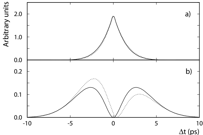
Figure 2.10: Time-dependent decay distributions for the final state D^{*-}\pi^{+} , for a) a \bar{B}^0 tag, and b) a B^0 tag. The situation with no doubly-CKM-suppressed contribution on both the reconstruction-side is indicated with the solid line. The dotted line has r = 0.1 , \delta = 0 , and 2\beta + \gamma = 1.86 . In these examples, r is 5 times the expected value in order to clearly illustrate the difference with respect to the case with r = 0 .
