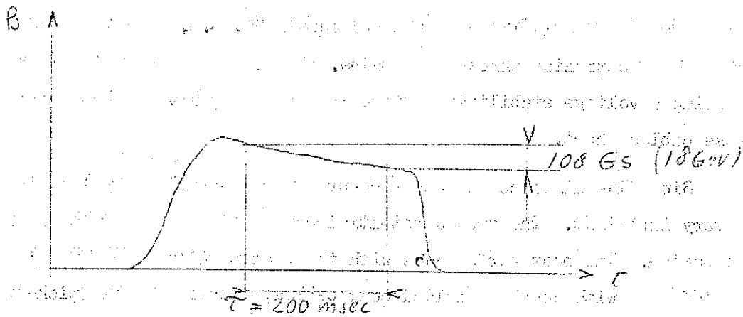
Fig. 1 Pulsed Magnet
