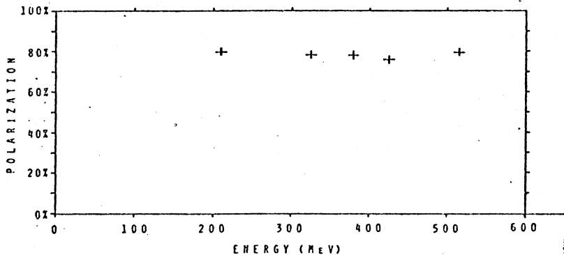
Fig. 2. Polarization of the extracted beam at various energies, measured by top scattering. There is ~6% uncertainty in the normalization; the statistical errors are smaller than the thickness of the lines.
