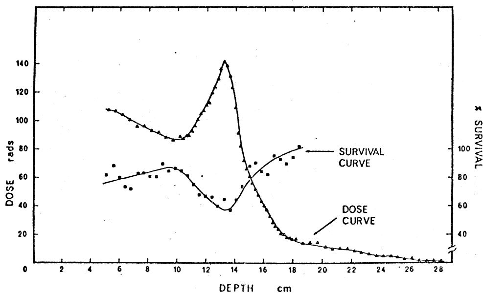
Fig. 6. \pi^- irradiation dose and cell survival expressed as a function of depth in water.
