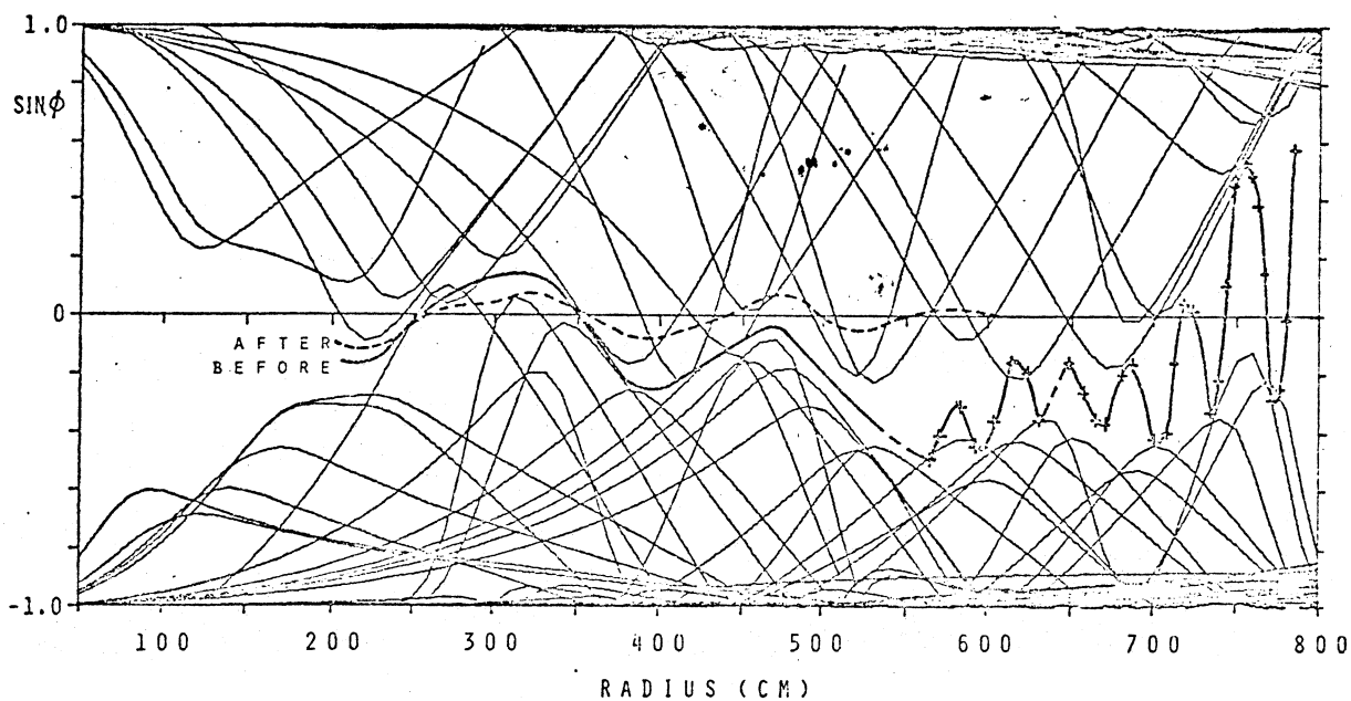
Fig. 4. Phase history \sin \phi(R) before (—) and after (---) the most recent adjustment of the 36 trim coils. The points (+) were obtained by timing external beams of different energies. The thinner peaked curves represent the phase changes induced by triplets of neighbouring trim coils needed to lose half the beam; the median phase curve should just touch them all.
