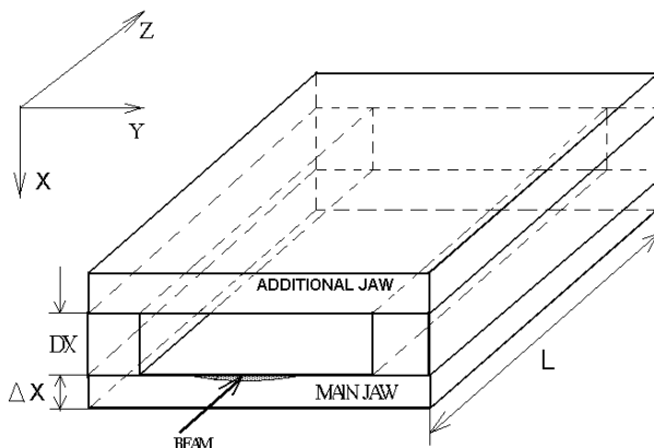
Fig.1: Rectangl collimator ( variant A ).
