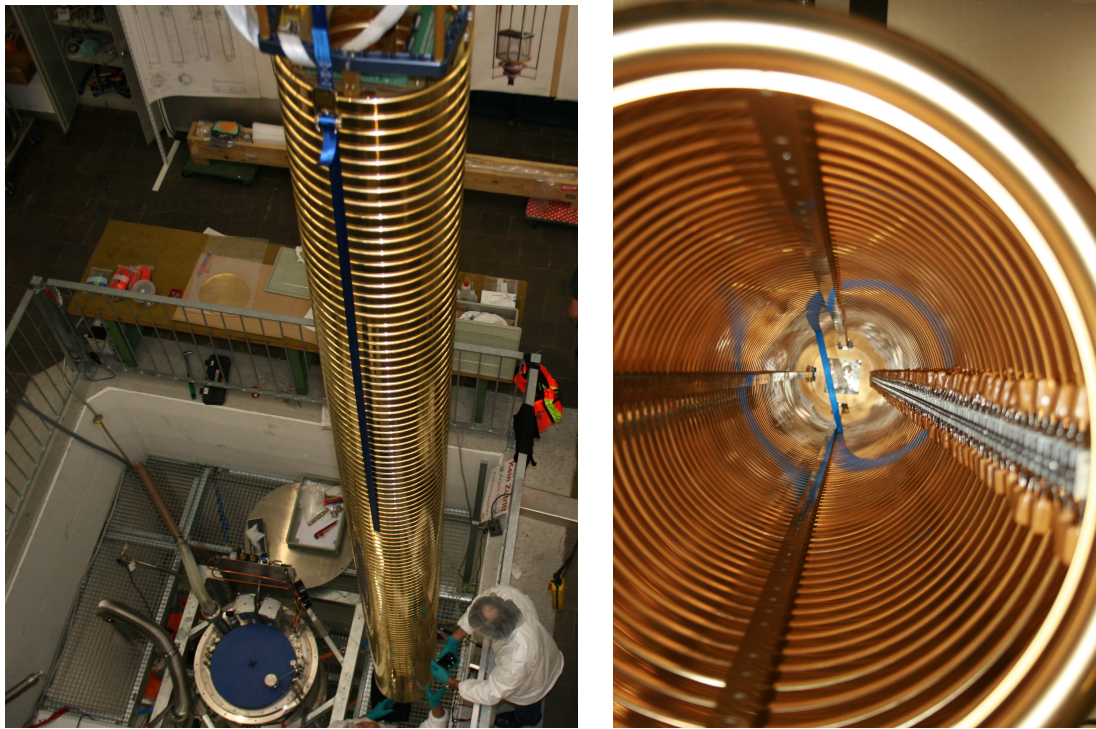
Figure 4. Left: Picture of the TPC with the 125 field shaping rings. Right: View inside the TPC with the mounted Greinacher/Cockcroft-Walton circuit visible on the side.
