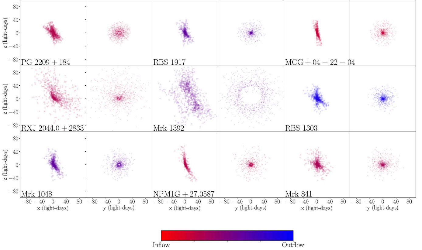
Figure 2. Geometric interpretation of BLR emission for the nine LAMP 2016 modelled sources using median parameter estimates. For each source, the left panel shows an edge-on view while the right panel shows a face-on view. Each circle corresponds to one point particle in the model. The geometries are color-coded to indicate whether the BLR dynamics exhibit inflow (red) or outflow (blue).
