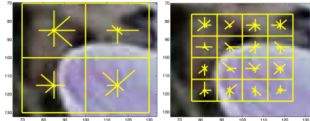
Fig. 3: Spatial binning of SIFT32 (left) vs SIFT128 (right)
