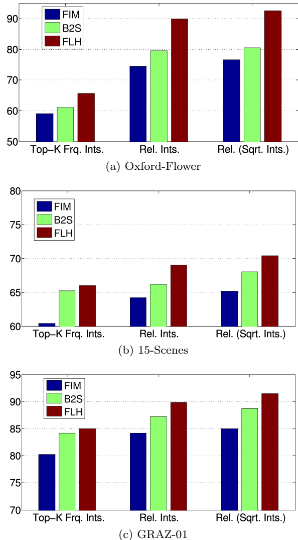
Fig. 8: Effect of larger spatial neighborhoods (25), smaller dictionary size (100) and SIFT-32 descriptor on frequent pattern-based image classification.
