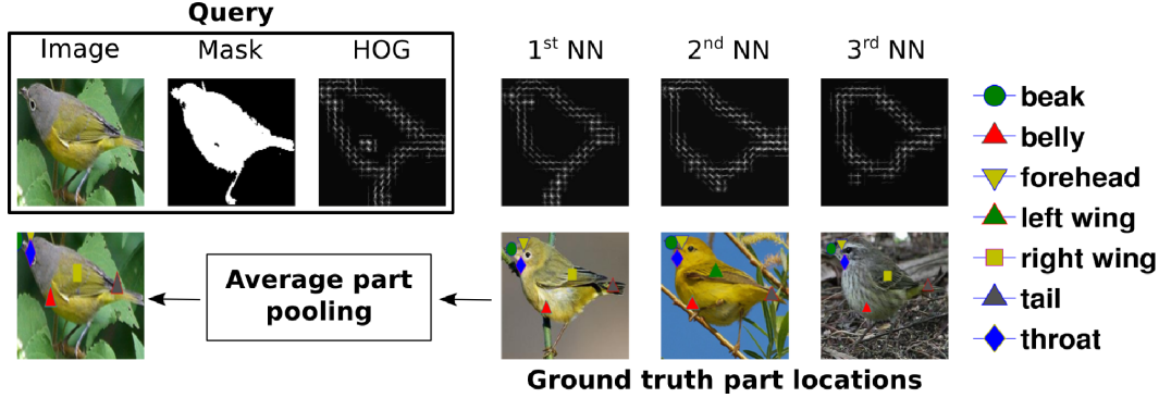
Figure 3. In the top left, we have a test image, for which we want to predict part locations. On the right, we have the nearest neighbor training images, their ground truth part locations and their HOG shape representations, based on which they were retrieved. Regressing the locations from the nearest neighbors to the test image we get the predicted parts, shown as the colorful symbols. The predicted part locations look quite consistent.
