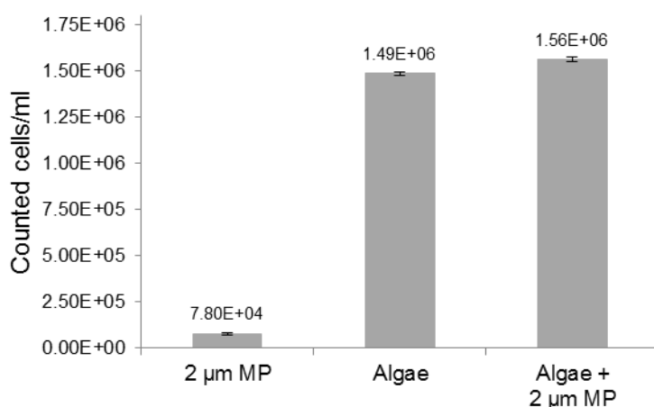
Fig. S8. Number of counted cells per ml in suspensions of 2 µm plastic particles (1 mg/l) and algal cells ( 1.5 \cdot 10^6 cells/ml) alone and in combination (n=3).
