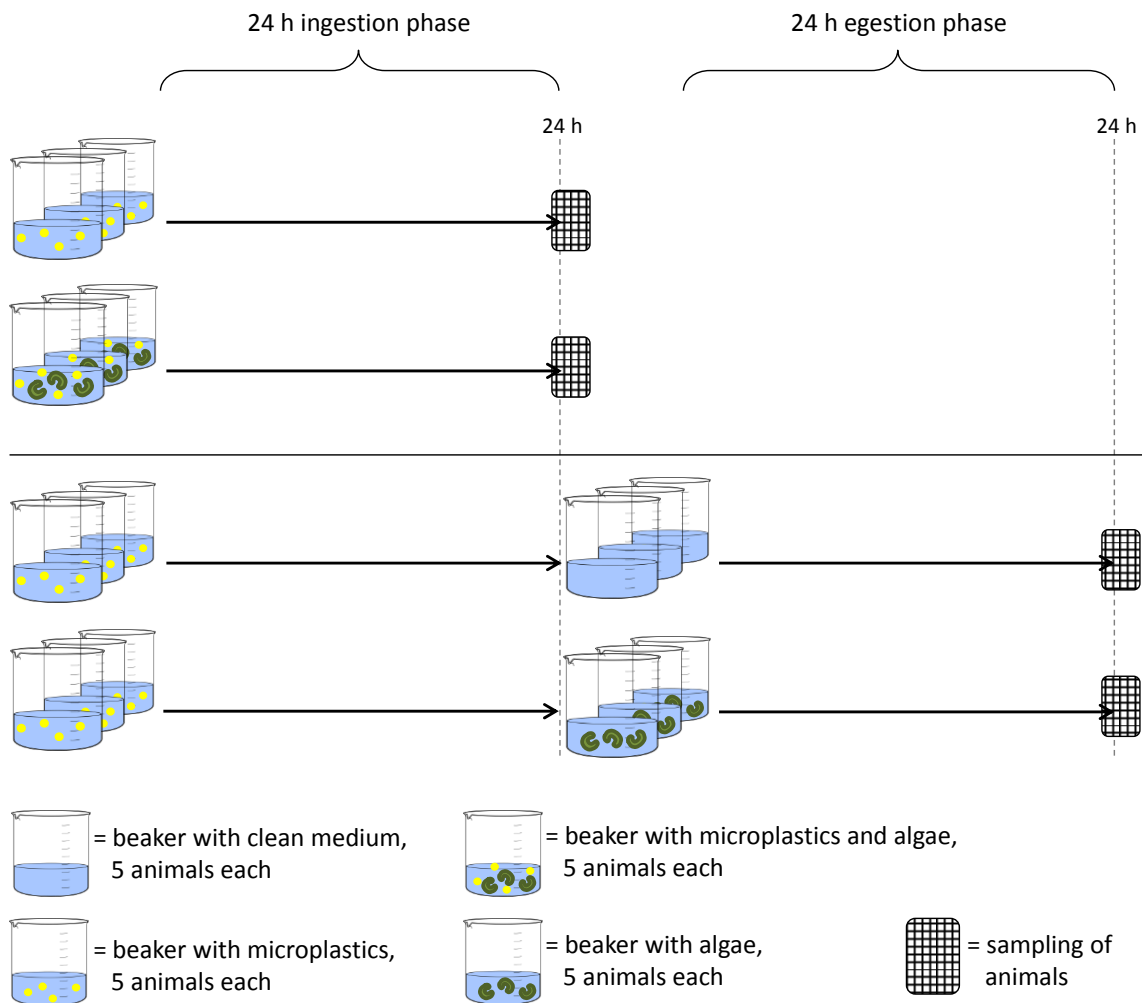
Fig. S2. Experimental design and setup of experiment 2. Daphnids were exposed to 1 mg/l of 100 nm or 2 \mu\text{m} particles (the figure only shows the setup for 1 particle size) with or without the addition of algae ( 6.7 \times 10^5 cells/ml) during a 24 h ingestion phase, followed by a 24 h egestion phase in clean medium, again with or without algae. Animals were sampled after 24 h, respectively. There were 5 one week old animals per beaker and 3 beakers per treatment group.
