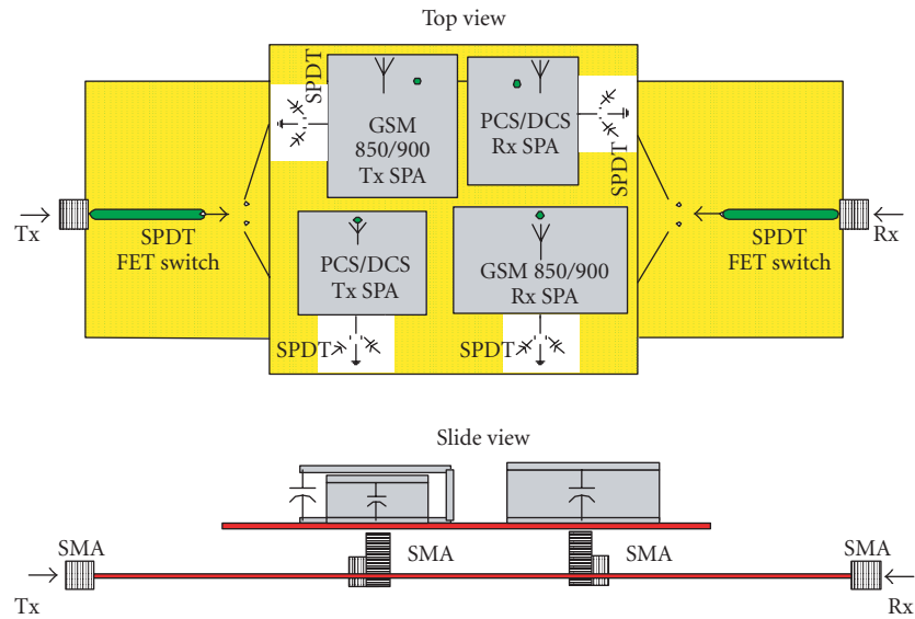
FIGURE 7: Prototype of tunable antennas for GSM850/900, DCS, and PCS.
