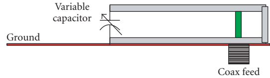
FIGURE 2: Geometry of SPA for reconfigurable antenna implementation.
