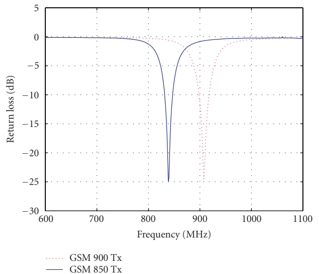
FIGURE 6: Measured return loss of the reconfigurable SPA between GSM 850 and GSM 900 bands.
