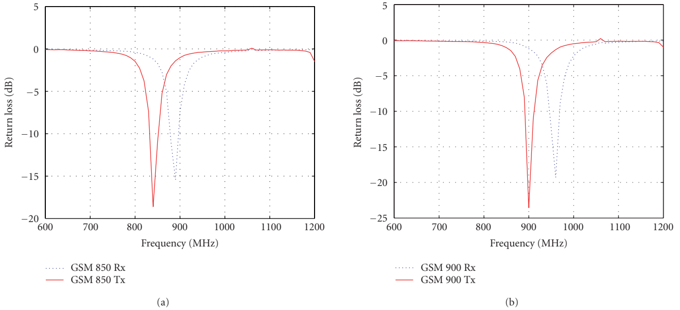
FIGURE 10: Measured return loss of tunable antenna pair tuned to (a) GSM 850 band and (b) GSM 900 band.
