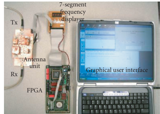
FIGURE 9: Test setup for demonstrating the electronically tunable antennas.
