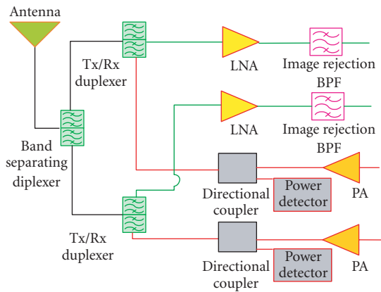
FIGURE 11: Conventional dual-band full-duplex RF front-end architecture.
