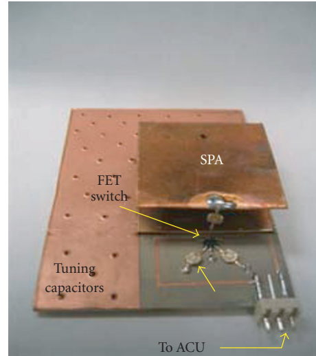
FIGURE 5: Photo of the fabricated tunable GSM 850/900 SPA.
