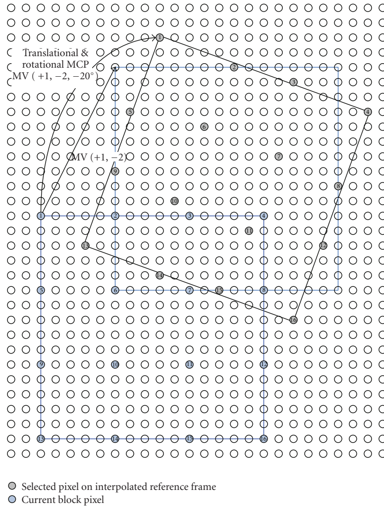
FIGURE 3: An example of translational and rotational MCP implemented by special subsampling on the interpolated reference frame.
